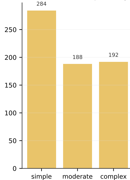
Formula complexity
