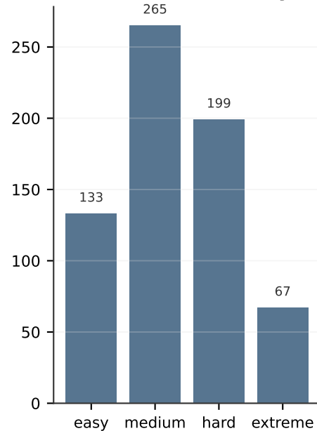
Probe4 difficulty
