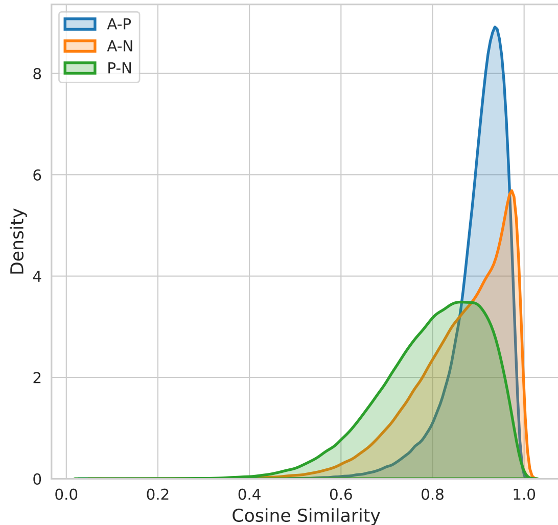
Semantic Similarity (Embedding Space)
