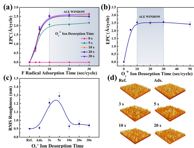
Figure 7. EPC of W ALE as a function of (a) F radical adsorption time and (b) O + ion desorption time. (c, d) Surface roughness after F radical adsorption and after the O + ion irradiation as a function of O + ion desorption, during the ALE of W. Reproduced with permission from [29], Copyright 2019, John Wiley and Sons.
