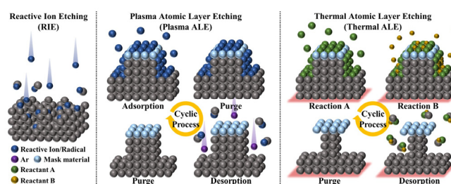
Figure 1. Comparison of RIE and anisotropic and isotropic ALE processes. ALE processes are cyclic processes that repeat adsorption reaction and desorption.
