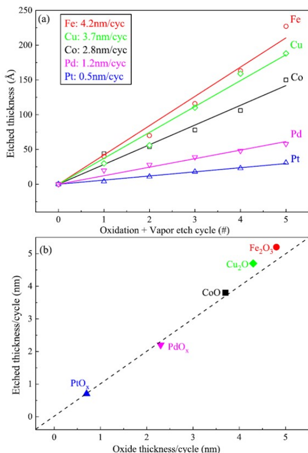
Figure 8. (a) Total etch depth as a function of ALE cycles and (b) EPC of different metal oxide thickness/cycle for anisotropic ALE of Co, Fe, Pd, Pt, and Cu, using O 2 plasma and formic acid. Reproduced with permission from [17], Copyright 2017, AIP Publishing.
