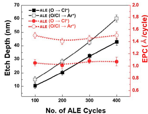
Figure 6. Total etch depth and EPC, measured as a function of the number of cycles by using physical (O/Cl radical adsorption and Ar + ion desorption) Cr ALE and chemical (O radical adsorption and Cl + ion desorption) Cr ALE. Reproduced with permission from [28], Copyright 2018, IOP Publishing.
