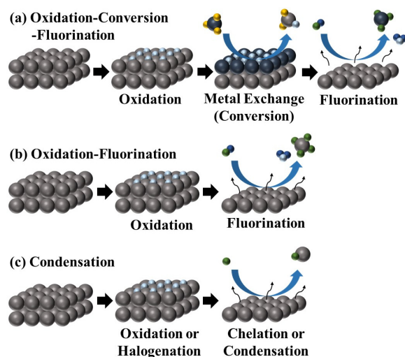
Figure 11. Thermal ALE methods capable of metal ALE.
