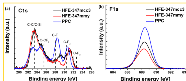
Figure 2. XPS spectra of fluorocarbon films on \text{SiO}_2 surfaces: (a) C 1s and (b) F 1s, derived from \text{n-C}_3\text{F}_7\text{OCH}_3 (HFE-347mcc3), \text{i-C}_3\text{F}_7\text{OCH}_3 (HFE-347mmy), and \text{CF}_3\text{CF}_2\text{CF}_2\text{CH}_2\text{OH} (PPC) plasmas. Reproduced with permission from [43], Copyright 2023, American Chemical Society.
