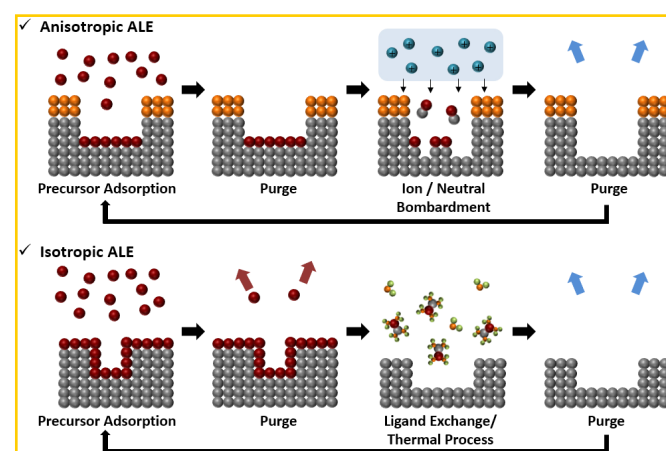
Figure 1. Comparative schematic of anisotropic and isotropic ALE processes for \text{SiO}_2
