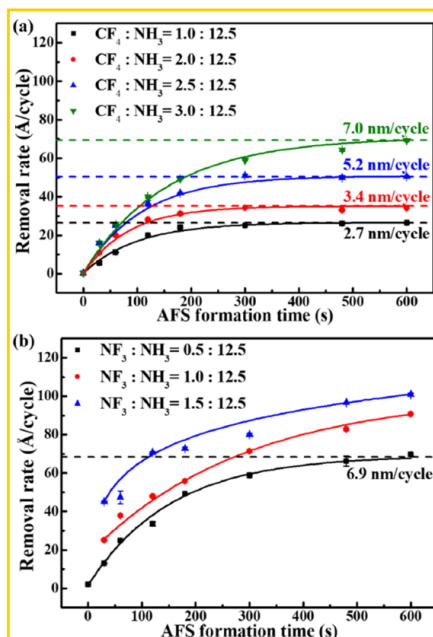
Figure 7. AFS formation time-dependent removal rates with (a) \text{CF}_4/\text{NH}_3 plasma and (b) \text{NF}_3/\text{NH}_3 plasma. Reproduced with permission from [35], Copyright 2020, AIP Publishing.
