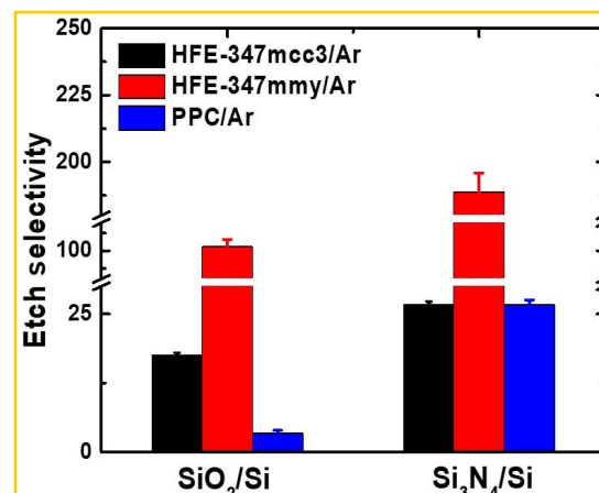
Figure 4. Precursor-dependent etching selectivity analysis for \text{SiO}_2/\text{Si} and \text{Si}_3\text{N}_4/\text{Si} in fluorination step. Reproduced with permission from [43], Copyright 2023, American Chemical Society.
