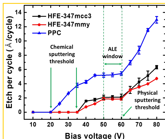
Figure 3. \text{SiO}_2 etching rates correlated with bias voltage in etching step, highlighting incomplete etching, ALE window, and physical sputtering regions based on ion energy. Reproduced with permission from [43], Copyright 2023, American Chemical Society.
