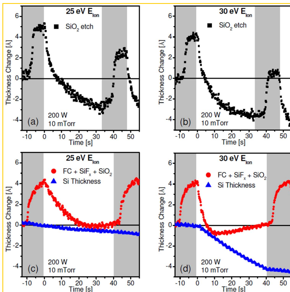
Figure 7. Time-dependent etching of \text{SiO}_2 and Si during one representative cycle each for \text{SiO}_2/\text{Si} based on \text{C}_4\text{F}_8/\text{Ar} ALE process. 100 In (a) and (b) deposition of FC on \text{SiO}_2 followed by etching at 25 eV and 30 eV maximum ion energy are shown, respectively, whereas in (c) and (d) deposition of FC on Si followed by etching at 25 eV and 30 eV maximum ion energy are shown, respectively. The most significant change is seen for the Si etch rate as the maximum ion energy is increased to 30 eV, leading to a very large increase of the Si etch rate, loss of self-limited etch rate and of \text{SiO}_2/\text{Si} etching selectivity.
