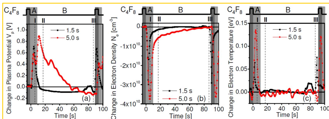
Figure 12. Evolution of plasma properties from cycle to cycle as measured using a Langmuir probe. 100 The cycle-to-cycle changes increase with C_4F_8 pulse length due to more residual FC in the system. This is explained by more deposition of FC on the walls of the apparatus, contributing residual FC during Ar cycles when ideally FC is only present on the active surface of the substrate. The overall behavior is consistent with the impact of continuous precursor addition on plasma electrical properties.
