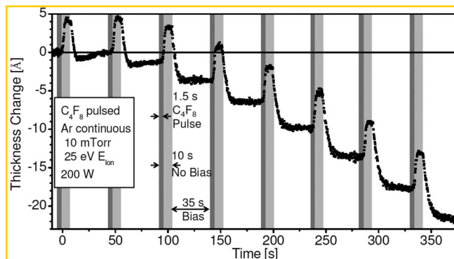
Figure 6. Example of thickness evolution during eight cycles of an \text{SiO}_2 ALE process. 99
