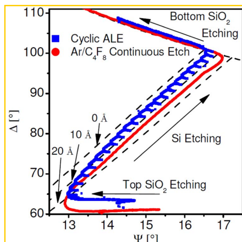
Figure 8. Real time ellipsometry trajectory showing key differences in surface processes between ALE and steady-state etching during continuous plasma etching of a \text{SiO}_2 -Si- \text{SiO}_2 multi-layer stack. 100 Each dashed line marks 10 Å of FC film.
