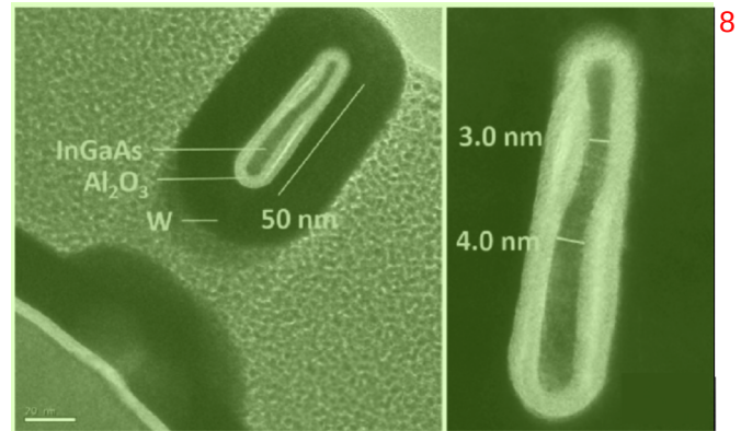
FIG. 8. TEM cross sections of a 4 \times 50 nm InGaAs nanowire covered by 4.7 nm ALD-grown \text{Al}_2\text{O}_3 and 20 nm of ALD tungsten. Reprinted with permission from Lu et al., in International Electron Devices Meeting, San Francisco, 1–5 December 2018 (IEDM, Montgomery Village, 2018), p. 895. Copyright 2018, IEEE.
