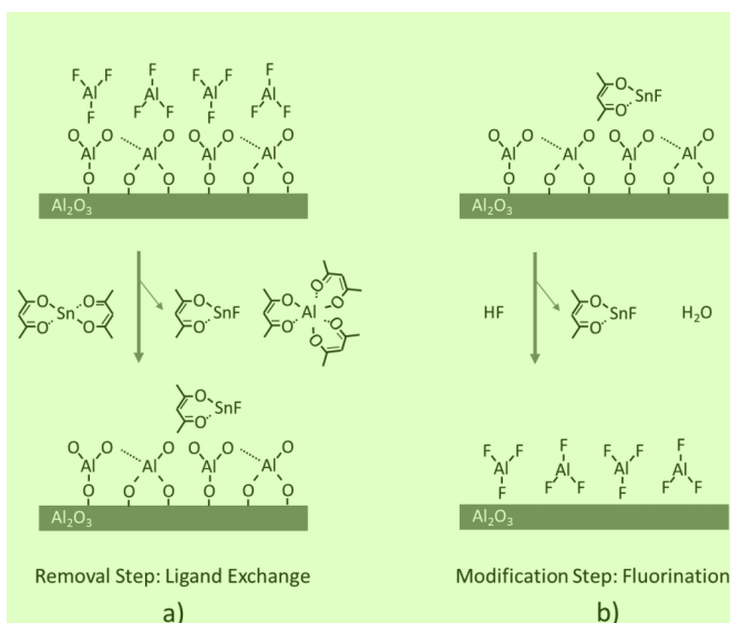
FIG. 4. Schematic of proposed reaction mechanism for \text{Al}_2\text{O}_3 ALE showing (a) \text{Sn}(\text{acac})_2 reaction and (b) HF reaction. Reprinted with permission from Lee and George, ACS Nano 9 , 2061 (2015). Copyright 2015, American Chemical Society.
