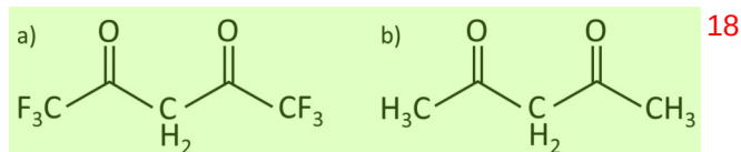
FIG. 2. Structural formulas of the keto tautomers of Hhfac (a) and Hacac (b).
