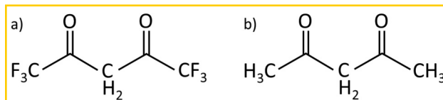
FIG. 2. Structural formulas of the keto tautomers of Hhfac (a) and Hacac (b).
