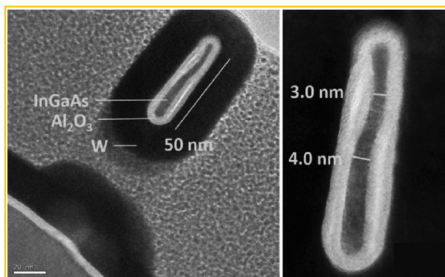
FIG. 8. TEM cross sections of a 4 \times 50 nm InGaAs nanowire covered by 4.7 nm ALD-grown \text{Al}_2\text{O}_3 and 20 nm of ALD tungsten. Reprinted with permission from Lu et al., in International Electron Devices Meeting, San Francisco, 1–5 December 2018 (IEDM, Montgomery Village, 2018), p. 895. Copyright 2018, IEEE.
