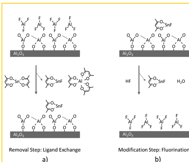
FIG. 4. Schematic of proposed reaction mechanism for \text{Al}_2\text{O}_3 ALE showing (a) Sn(acac) 3 reaction and (b) HF reaction. Reprinted with permission from Lee and George, ACS Nano 9 , 2061 (2015). Copyright 2015, American Chemical Society.
