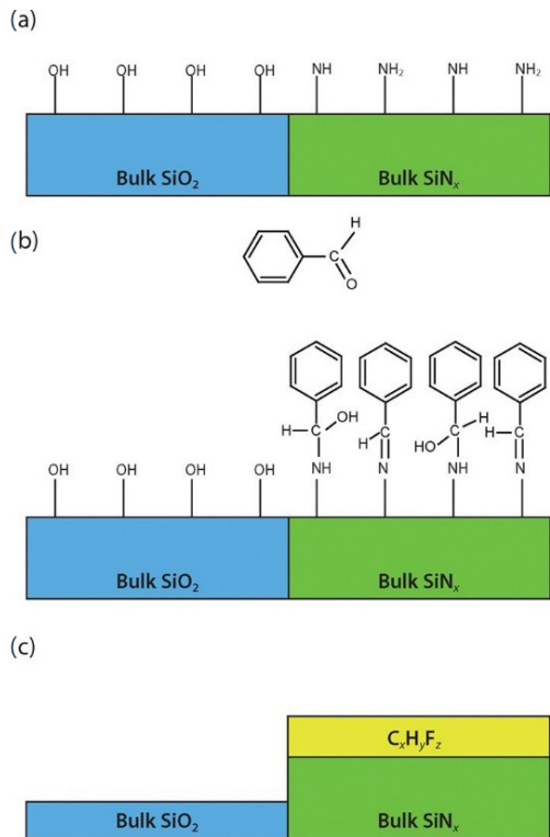
Figure 5. Selective ALE process of \text{SiO}_2 over \text{SiN}_x : (a) Initial functional groups on plasma-deposited surfaces; (b) selective functionalization of \text{SiN}_x surface with benzaldehyde; (c) aromatic aldehyde aiding graphitic hydrofluorocarbon film formation on \text{SiN}_x surface during ALE, inhibiting \text{SiN}_x etching. Reproduced with permission from [38], Copyright 2021, AIP Publishing.
