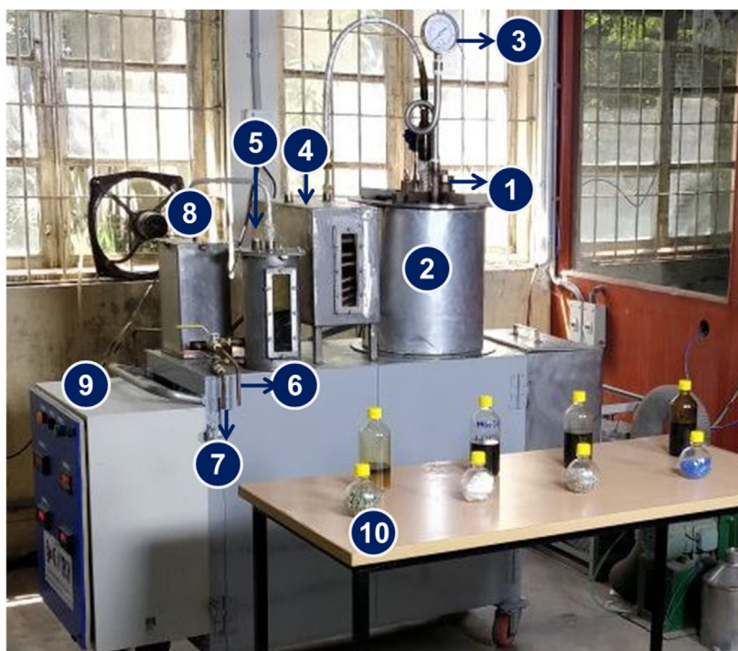
Components: 1. Feed Inlet; 2. Pyrolysis chamber; 3. Pressure gauge; 4. Condenser I; 5. Condenser II and oil collection system; 6. Pyrolysis oil collection valve; 7. Water disposal valve; 8. Gas scrubber unit; 9. Controller unit; 10. Pyrolysis oil collected for different types of plastics
