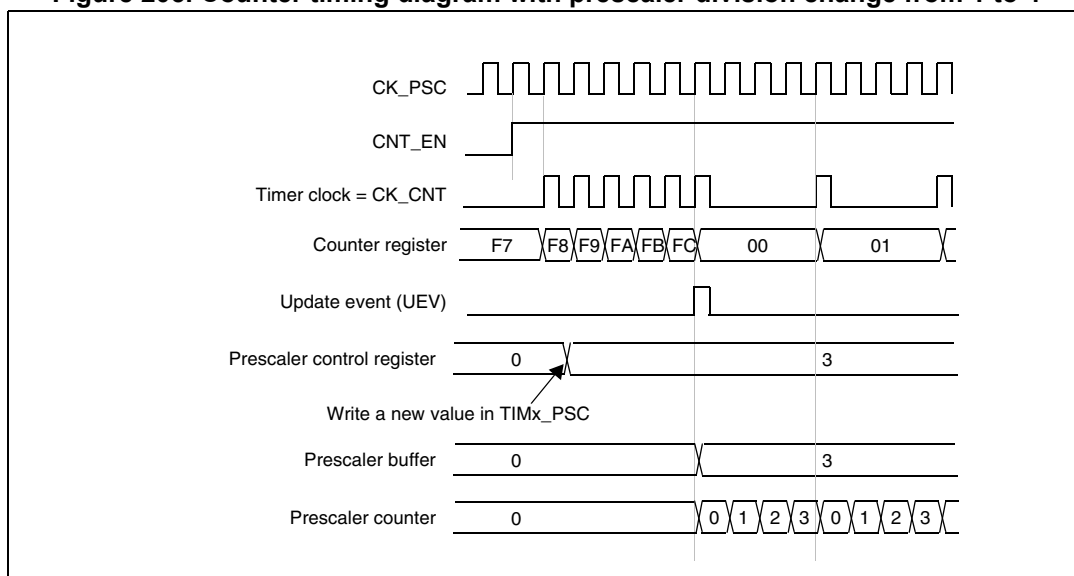
Figure 205. Counter timing diagram with prescaler division change from 1 to 4
