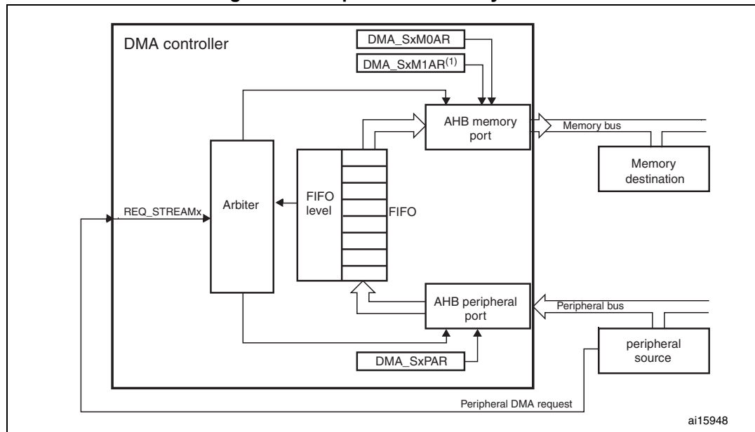
Figure 36. Peripheral-to-memory mode
