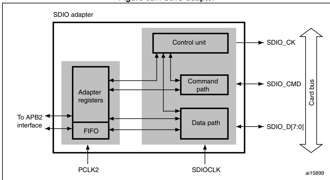
Figure 327. SDIO adapter
