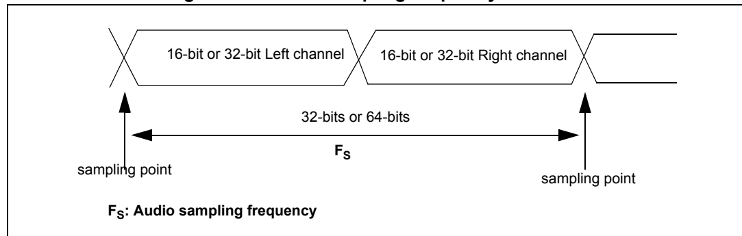
Figure 281. Audio sampling frequency definition
