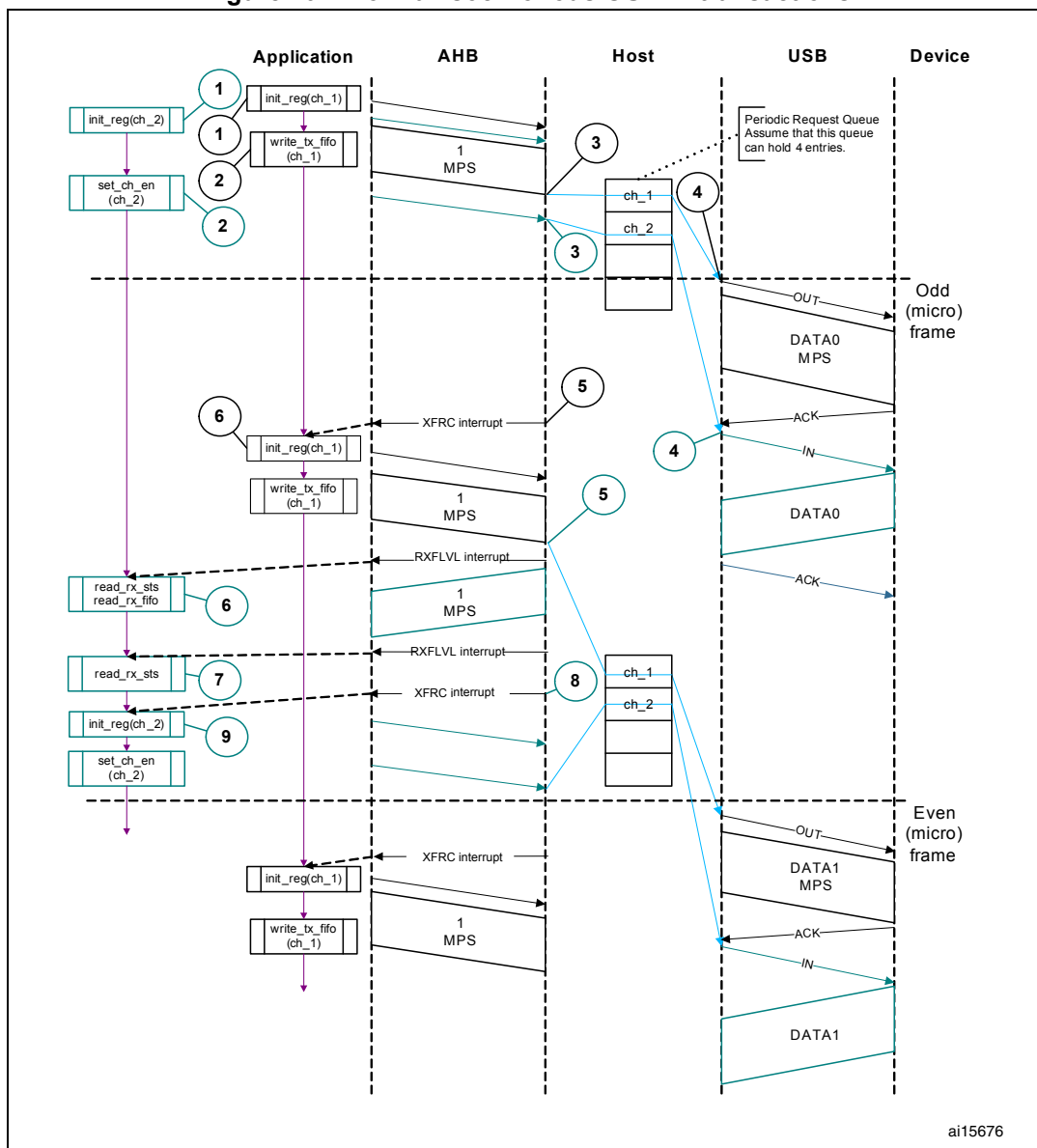
Figure 401. Normal isochronous OUT/IN transactions
