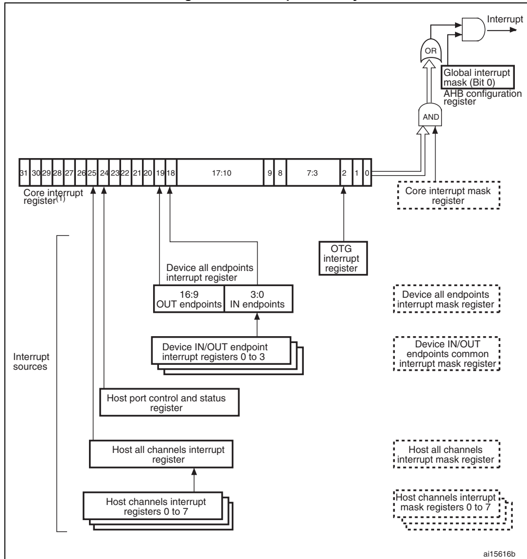
Figure 394. Interrupt hierarchy
