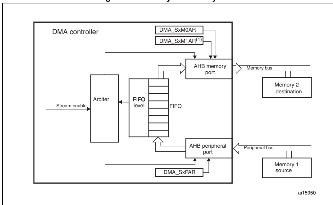
Figure 38. Memory-to-memory mode
