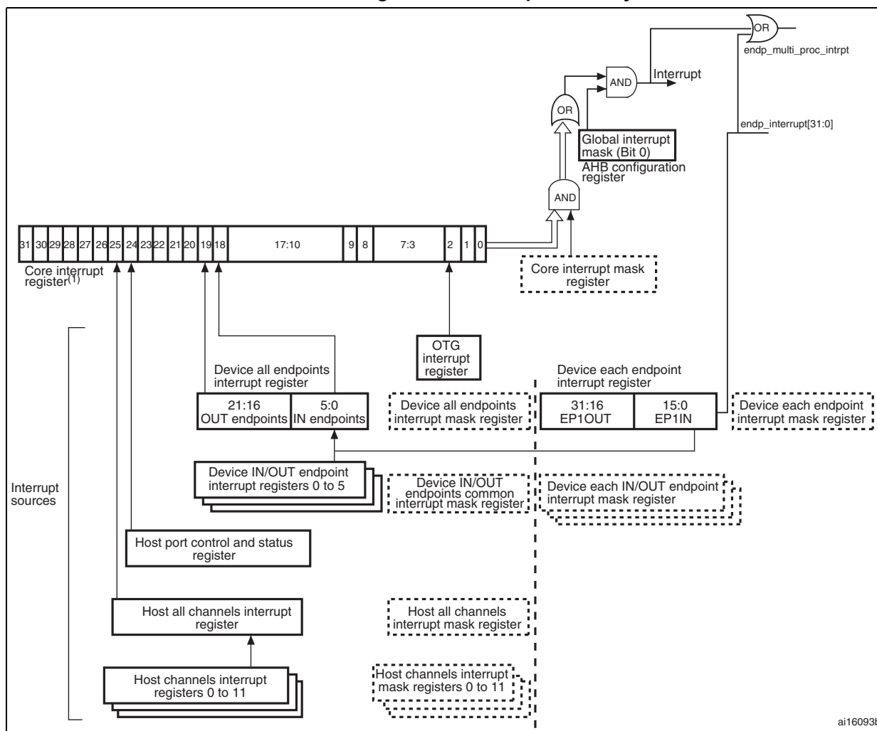
Figure 412. Interrupt hierarchy
