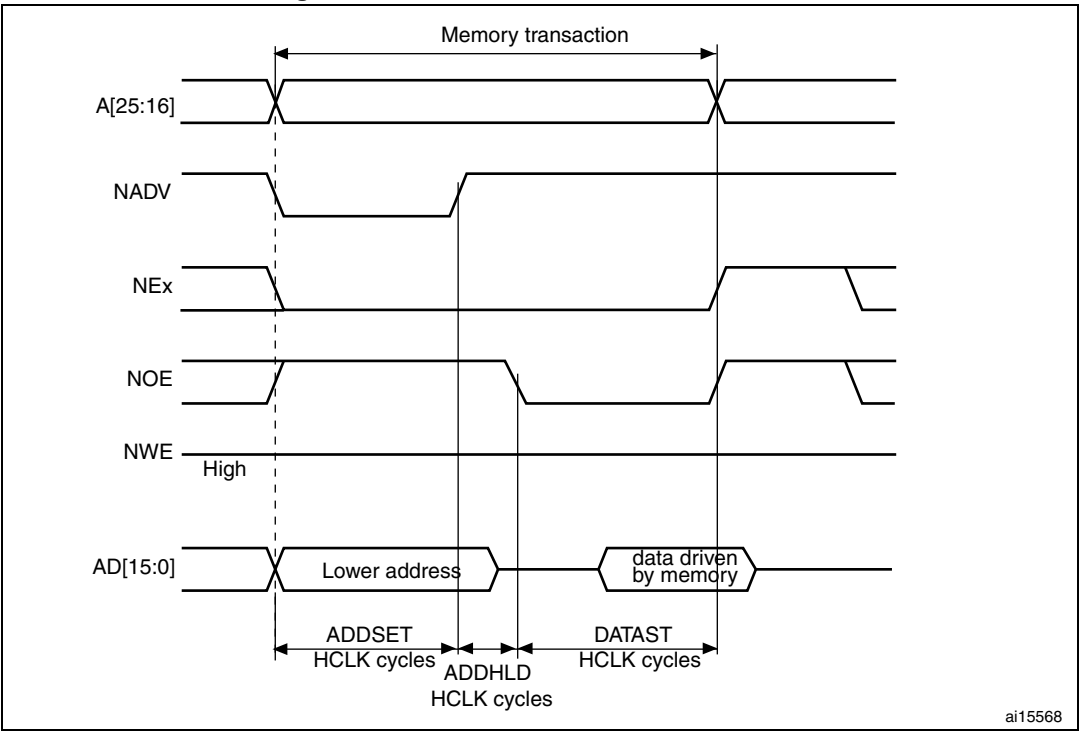
Figure 467. Muxed read access waveforms
