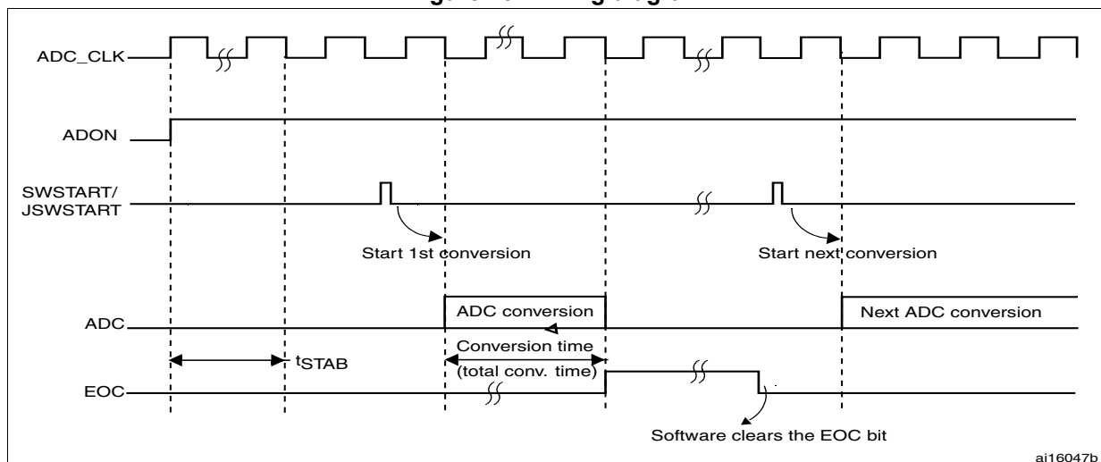
Figure 45. Timing diagram
