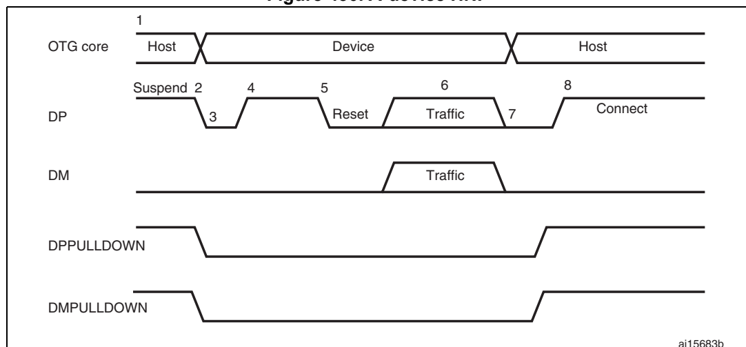
Figure 430. A-device HNP
