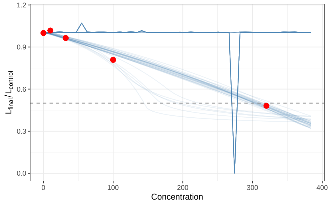
DEBtox Dose-Response (full model prediction)
