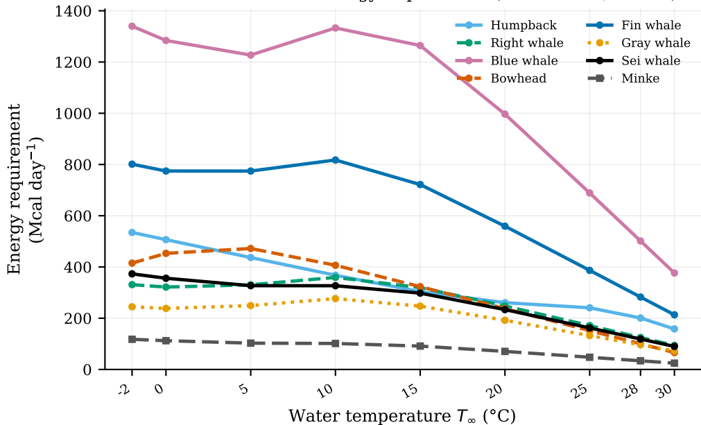
Thermal-maintenance energy requirement (active mode, FA = 1)
