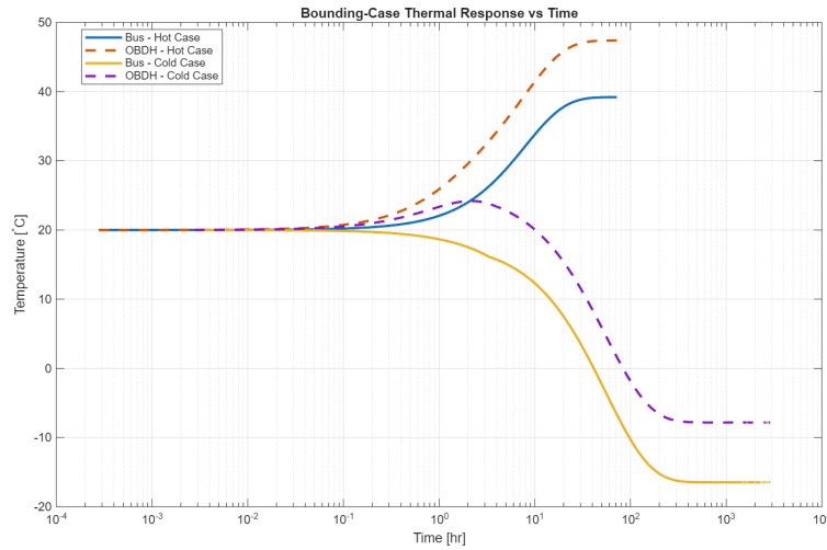
Fig. 7 Transient hot- and cold-case temperature response of the spacecraft bus and critical OBDH node. The hot case assumes a fixed perihelion environment at 0.046 AU, while the cold case assumes deep-space conditions near 900 AU. The curves show the time required for each node to approach thermal equilibrium under these bounding conditions.
