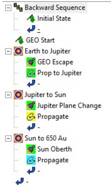
Fig. 15 Astrogator Mission Control Sequence (MCS) for the Destiny trajectory.
