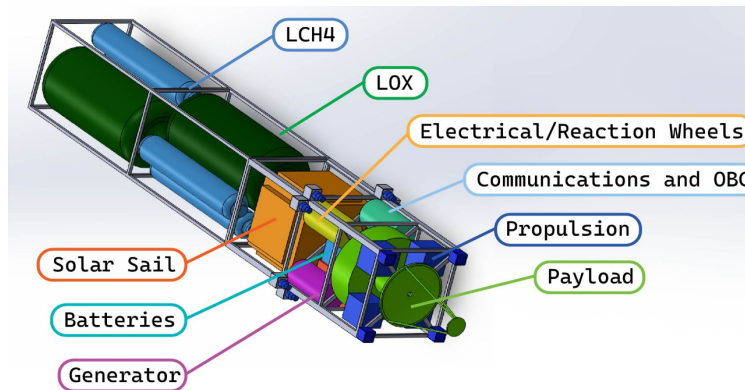
Fig. 4 All stages of the spacecraft
