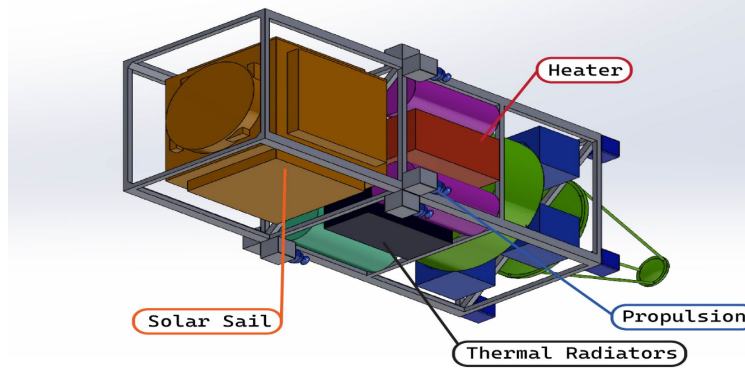
Fig. 5 Final Stage of the spacecraft
