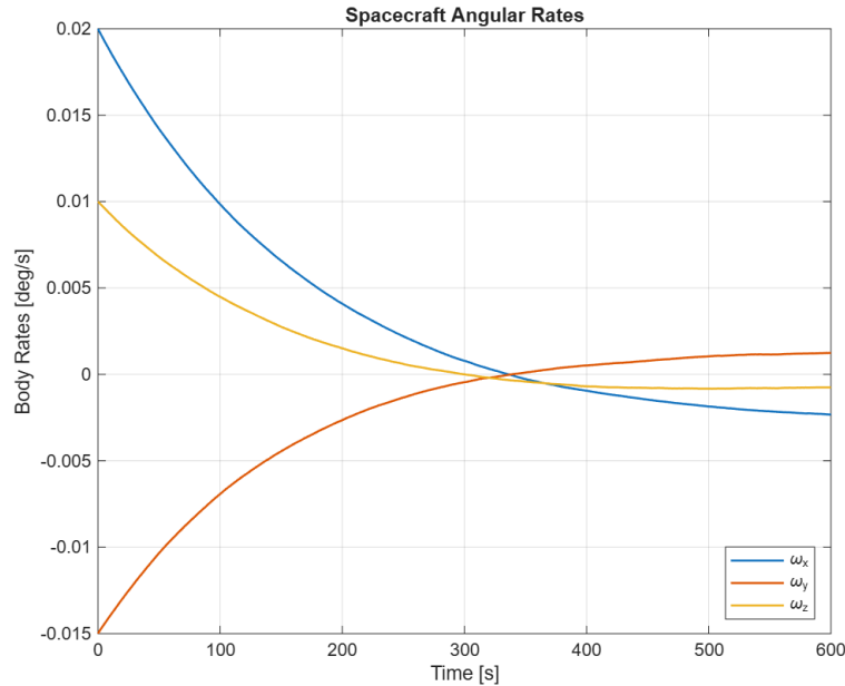
Fig. 9 The simulation incorporates the concept of the TRIAD (Tri-Axial Attitude Determination) method, which utilizes body-frame vectors derived from star tracker centroid measurements. These vectors are compared to known inertial reference vectors from onboard star catalogs to determine the spacecraft's orientation.
