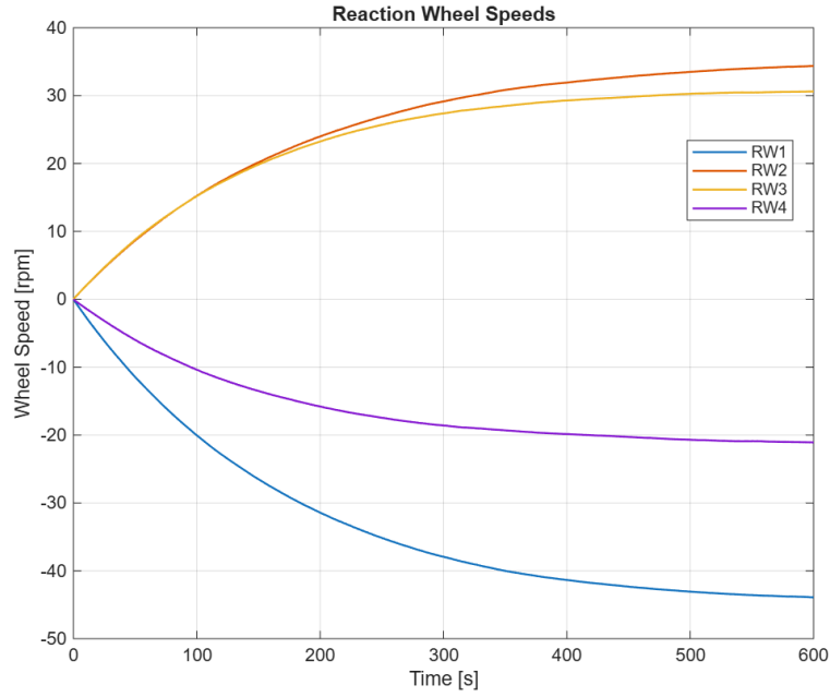
Fig. 10 Reaction wheels generate controlled torques by varying their individual rotational speeds, enabling smooth and continuous attitude adjustments without the use of propellant.
