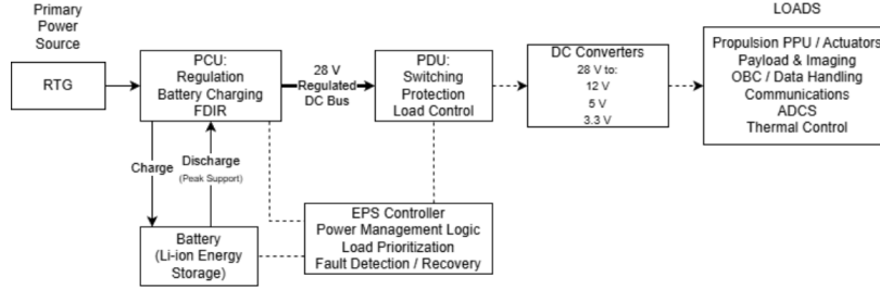
Fig. 13 Diagram of EPS subsystem Link
