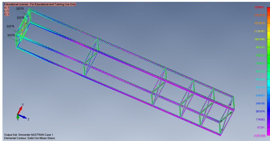
Fig. 18 FEMAP Plot of Von Mises Stress
