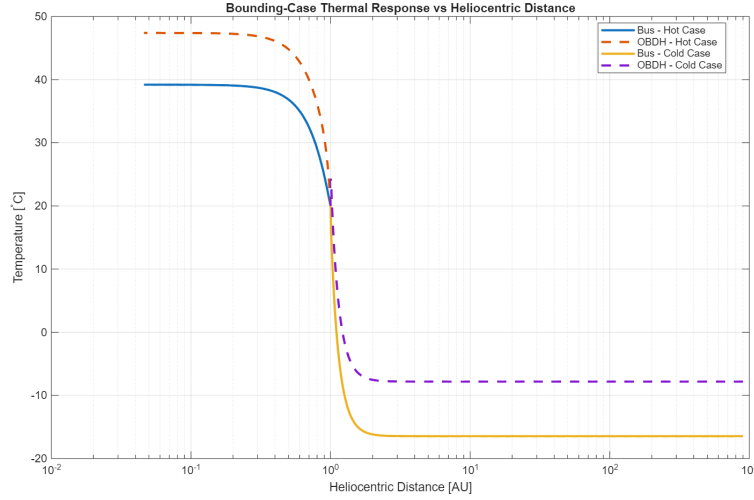
Fig. 8 Bounding-case thermal response of the spacecraft bus and critical OBDH node plotted against representative heliocentric distance. The hot- and cold-case results are shown over their respective distance ranges to illustrate thermal behavior near perihelion and in deep-space conditions. This figure does not represent a continuous trajectory simulation.
