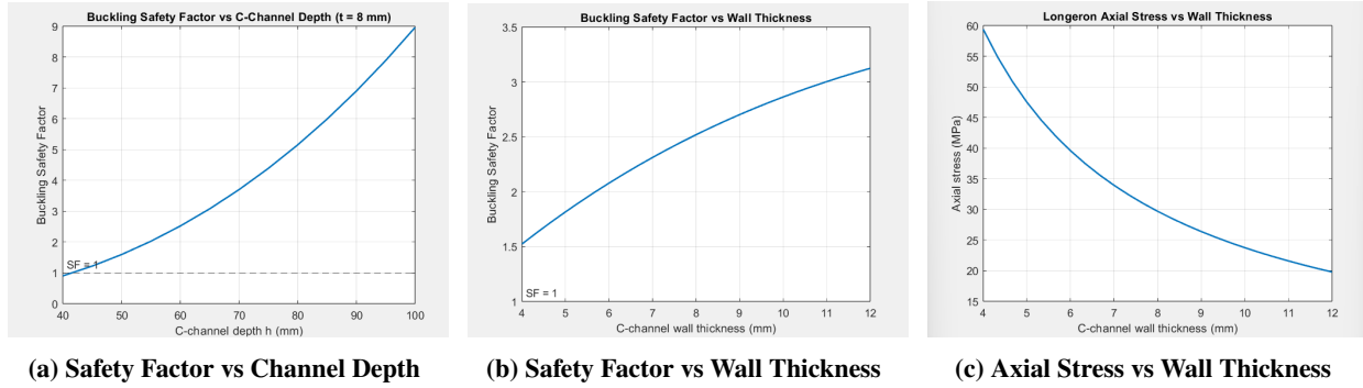
Fig. 17 Structural response metrics as a function of channel depth and wall thickness
