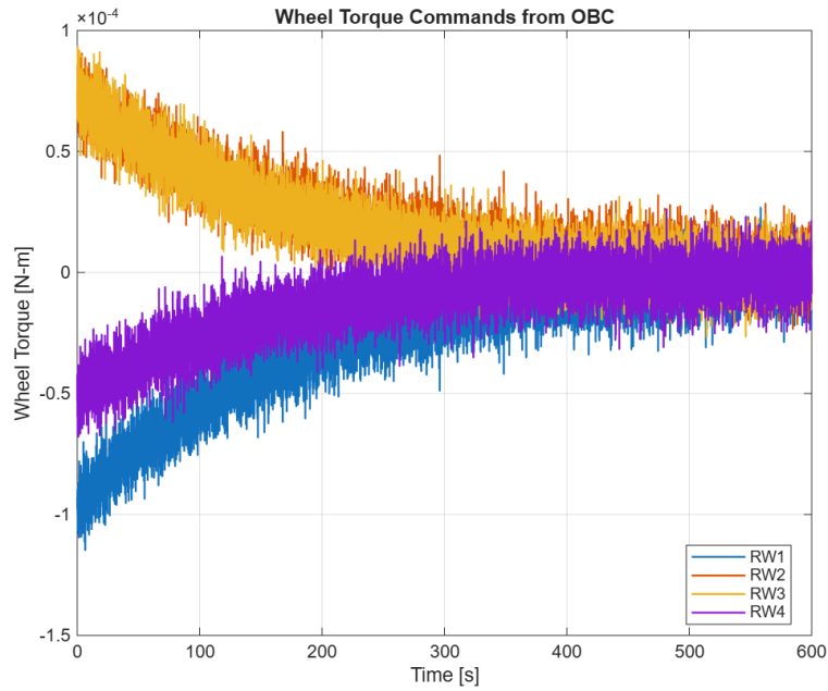
Fig. 11 The On Board Computer (OBC) is in this case is responsible for mainly Processing sensor data, running attitude determination algorithms (e.g., TRIAD-based methods), computing control commands and distributing torque commands to reaction wheels.
