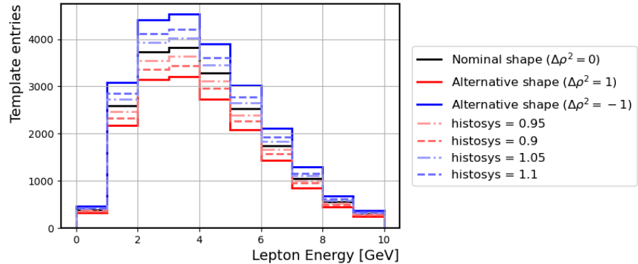
Figure 3. Distributions of a 1-dimensional pyhf template for different values of the histosys modifier, defined with respect to two different injection of values of the \rho^2 FF parameter in HAMMER. Redist-HAMMER allows the integration of the theoretical uncertainty on the Form Factor parameter as a standard histosys nuisance parameter in pyhf .
