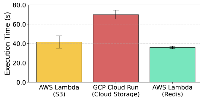
Figure 3. TeraSort performance of Lithops across different cloud providers and storage backends (in parentheses).
