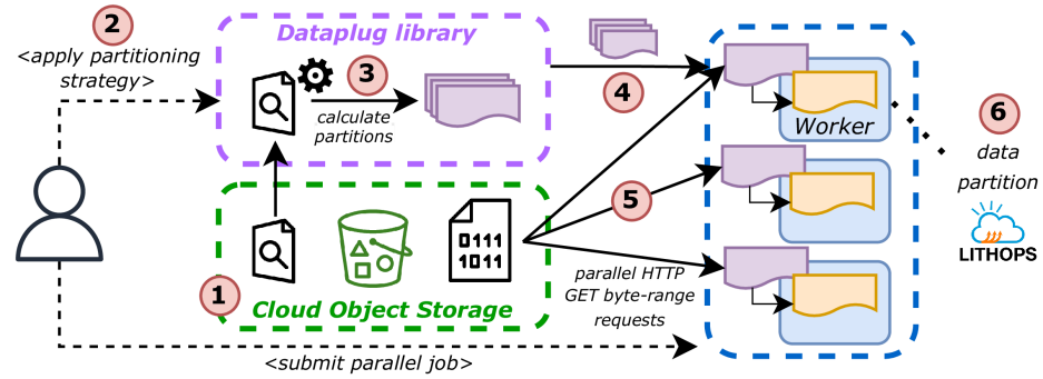
Figure 5. Dataplug workflow.
