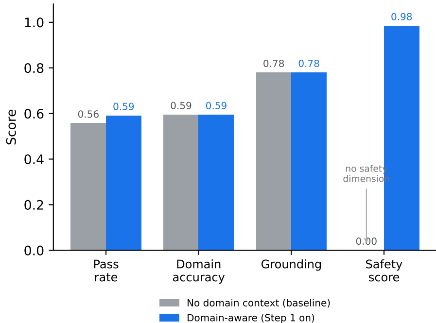
(a) FinanceBench: scored metrics (our run, baseline vs domain-aware)
