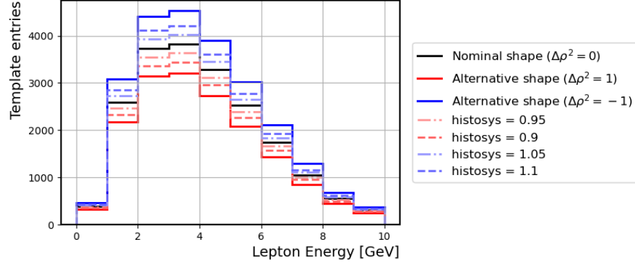
Figure 2. Distributions of a 1-dimensional pyhf template for different values of the histosys modifier, defined with respect to two different injection of values of the \rho^2 FF parameter in HAMMER.
