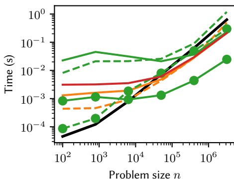
scipy.spatial.transform.Rotation.mean
