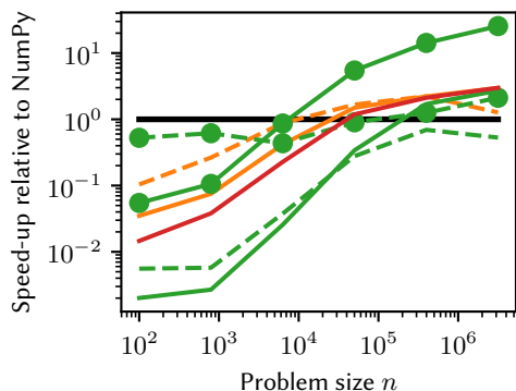
scipy.spatial.transform.Rotation.mean
