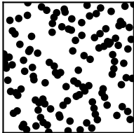
D) LHS
