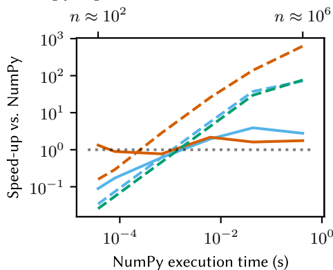
c) scipy.spatial.transform.Rotation.mean
