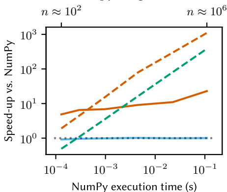
c) scipy.spatial.transform.Rotation.mean
