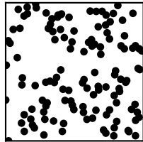
A) IID uniform
