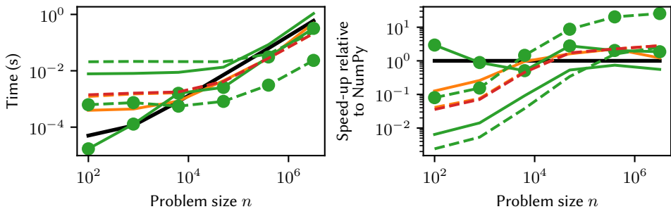
c) scipy.spatial.transform.Rotation.mean
