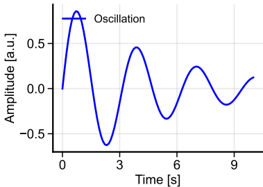
Damped Oscillation (Custom Style)
