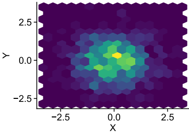
mpl_hexbin
