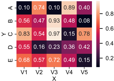
sns_heatmap
