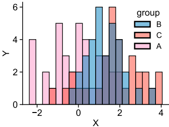
sns_histplot
