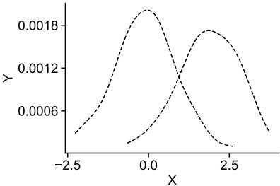
sns_kdeplot
