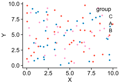
sns_scatterplot
