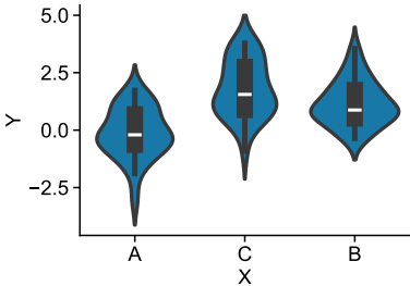
sns_violinplot
