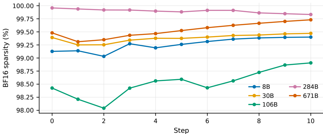
Figure 7: BF16 element-level sparsity across five models spanning 8B to 671B parameters over synchronization steps. All models exhibit high sparsity ( \geq 98\% ) from the first step, and for most of them sparsity tends to increase over training. The 284B model (DeepSeek-V4-Flash, the most recent generation) is the sparsest at every step ( > 99.8\% throughout); among the older-generation models the 671B reaches the highest level, consistent with larger pretrained weights having more mass in the sub-threshold regime that gets absorbed by the BF16 cast.
