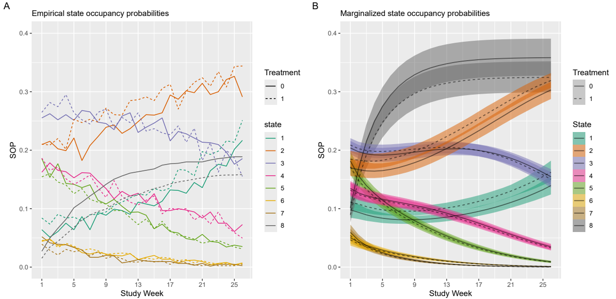
Figure 11: Comparison of empirical SOPs (A) vs. model-derived SOPs using interval censoring (B). The model significantly overestimates the cumulative incidence of death (State 8).
