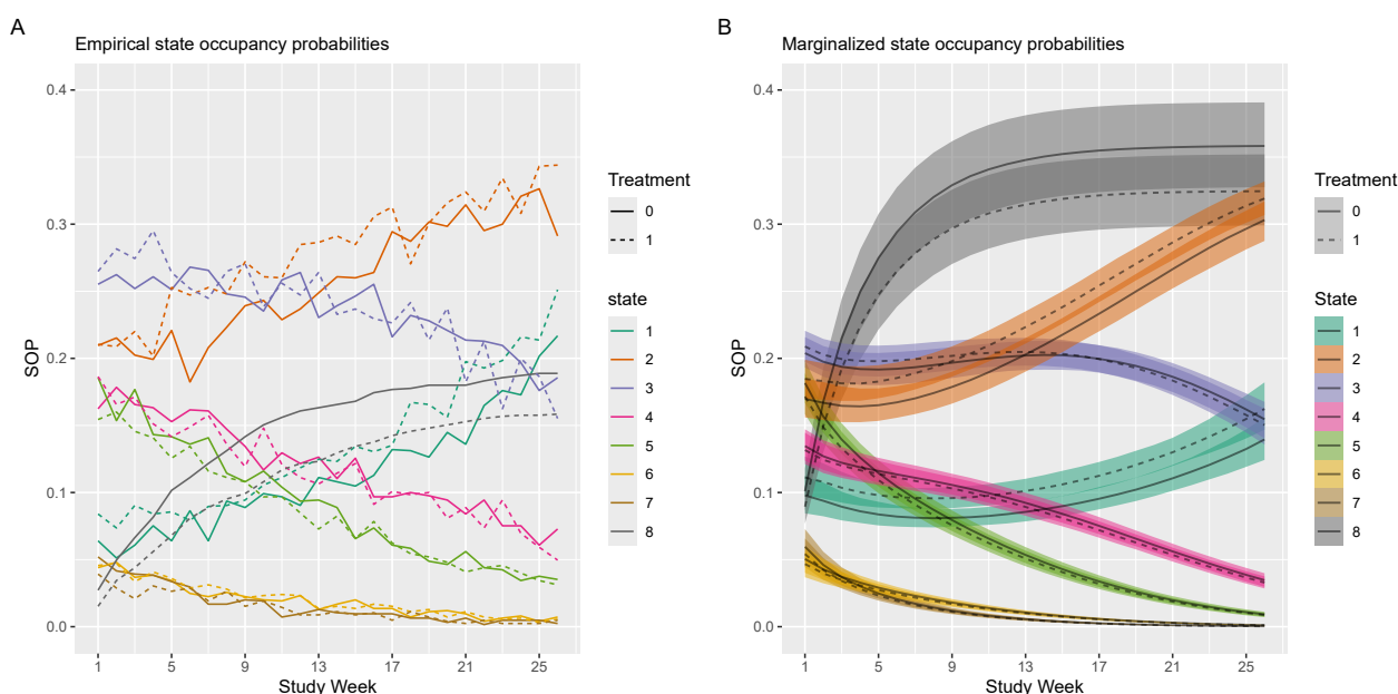
Figure 31: Comparison of empirical SOPs (A) vs. model-derived SOPs using interval censoring (B). The model significantly overestimates the cumulative incidence of death (State 8).
