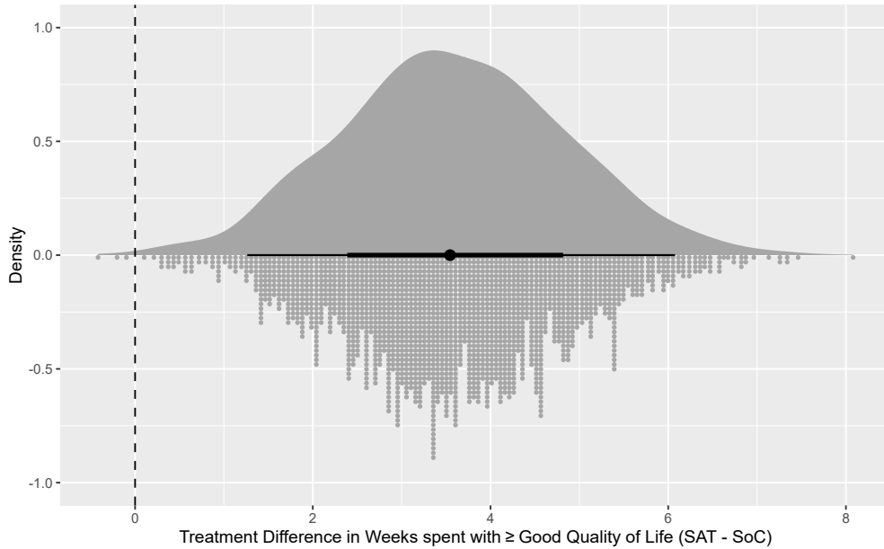
Figure 5: Posterior distribution of the estimated difference in weeks with good or better quality of life ( \hat{\tau}_{QoL} ), defined as state 1, 2, or 3, based on a sample ( n = 216 ) of simulated data with a true underlying difference of two weeks. Larger values favour the group selected for invitation to the SAT.
