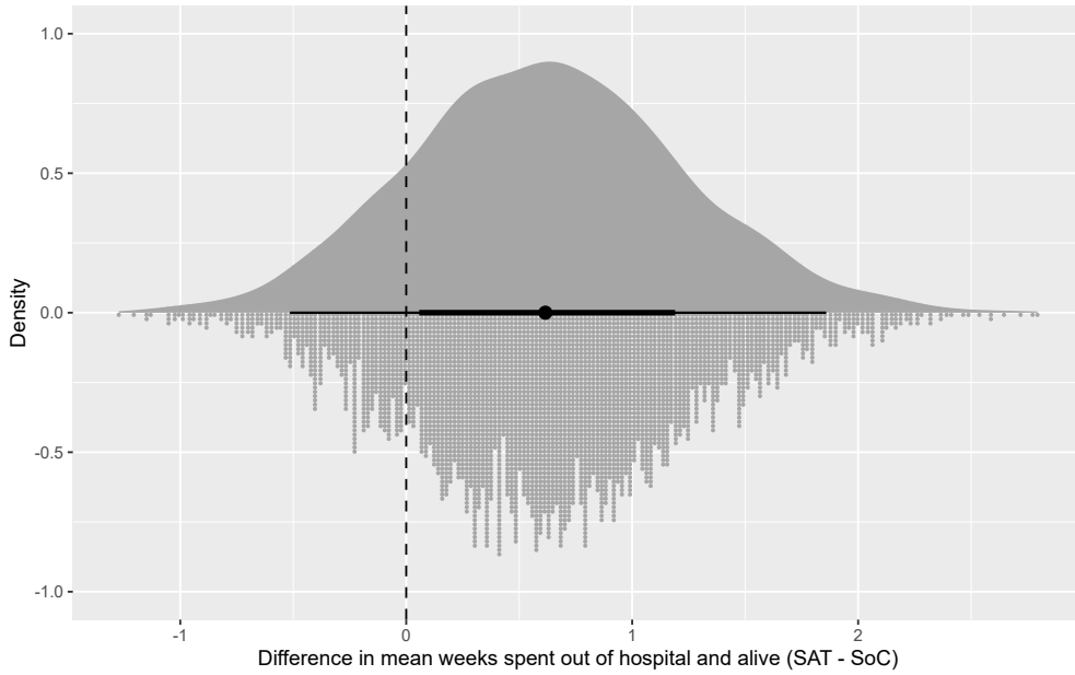
Figure 9: Posterior distribution of the primary estimand, the expected difference in weeks alive and out of hospital ( \hat{\tau}_{TAOOH} ), defined as state 1, based on a sample ( n = 270 ) from simulated data with a true underlying OR = 0.8 for transitioning to a worse state for the group selected for invitation to the single-arm trial ( \tau \approx 1.2 weeks). Larger values favour the group invited to the SAT.
