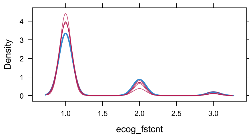
Figure 21: Density plot for ECOG performance status.
