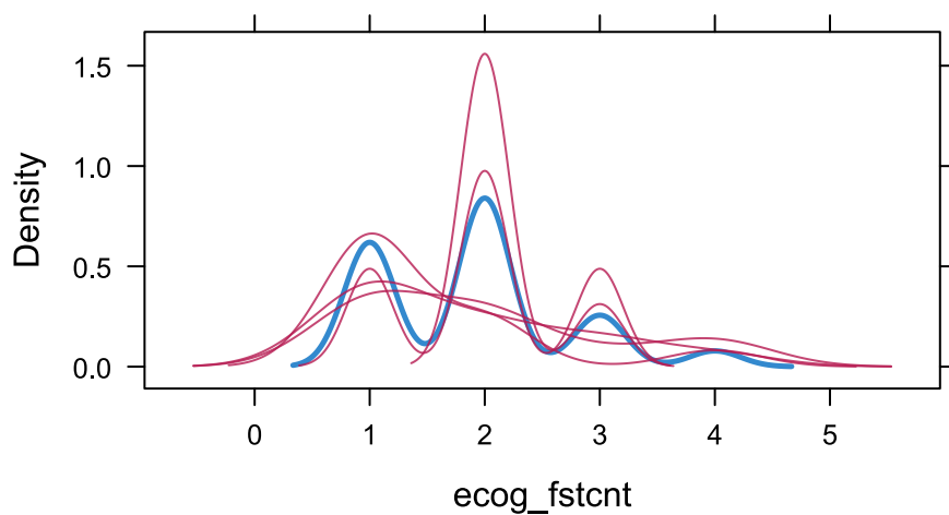
Figure 27: Density plot for ECOG performance status.
