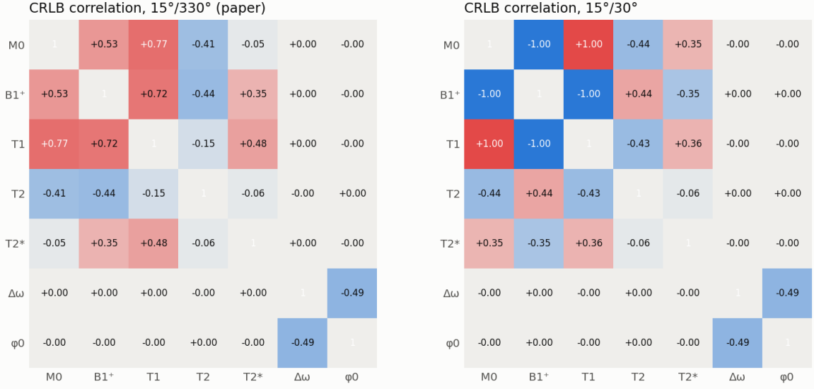
Figure 1: Correlation matrices of the CRLB covariance \mathcal{I}^{-1} . Right: the M_0 - B_1^+ - T_1 block of the small-angle protocol is perfectly correlated, the signature of the invariance (17).
