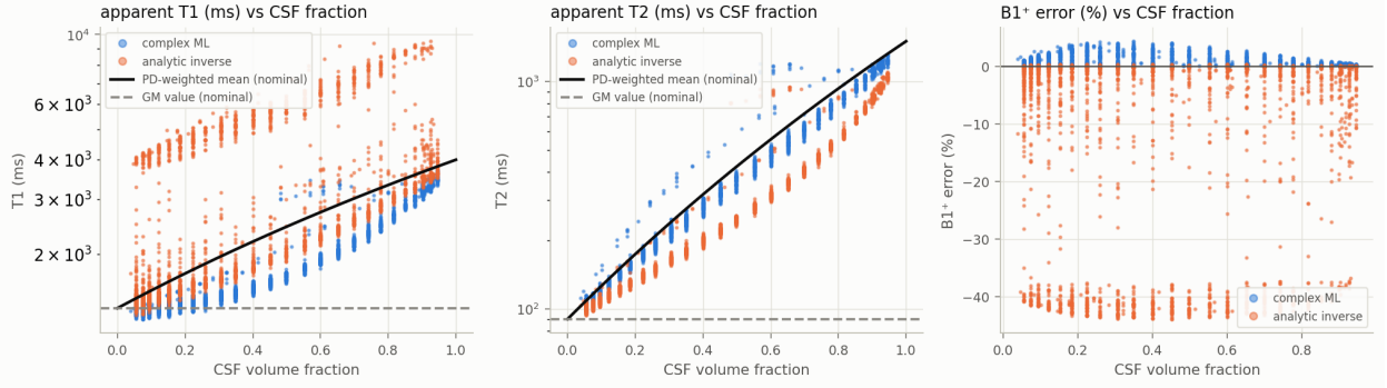
BrainWeb GM/CSF voxels, noise-free: the single-compartment fit of a mixture
