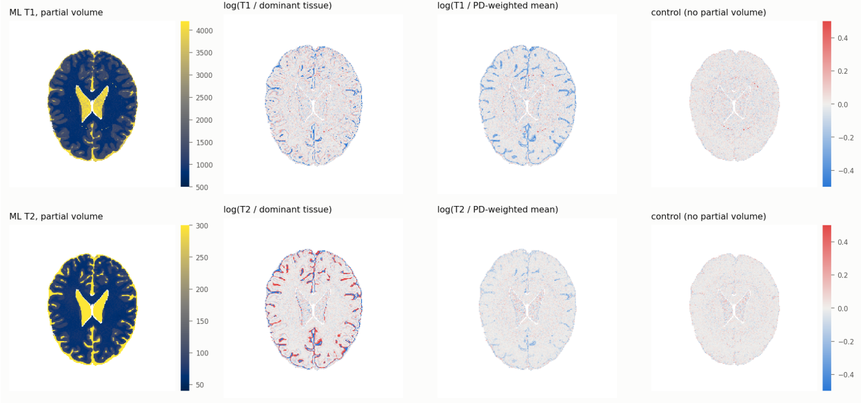
Figure 18: Complex ML at \text{SNR}(M_0) = 1000 . From left: estimate with partial volume; log-ratio to the dominant tissue’s value; log-ratio to the PD-weighted mean; the same anatomy without partial volume (control). Rows: T_1 and T_2 .
