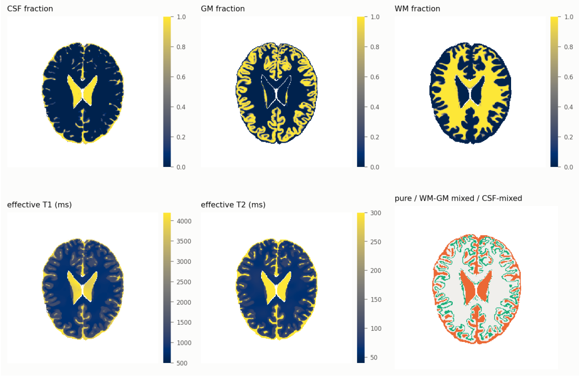
Figure 16: BrainWeb slice: tissue fractions, the PD-weighted effective T_1 and T_2 , and voxel categories (pure; WM/GM mixed; containing \geq 5\% CSF).
