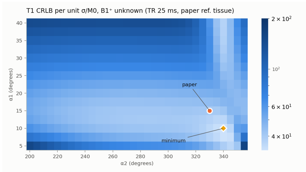
Figure 5: T_1 bound with B_1^+ unknown over nominal (\alpha_1, \alpha_2) .
