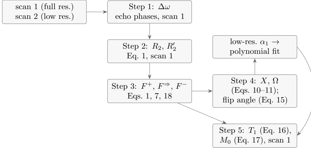
Figure 3: The published reconstruction [1]. The flip angle is computed at the resolution of scan 2 and smoothed by a polynomial; T_1 and M_0 are then computed voxel-wise from scan 1.
