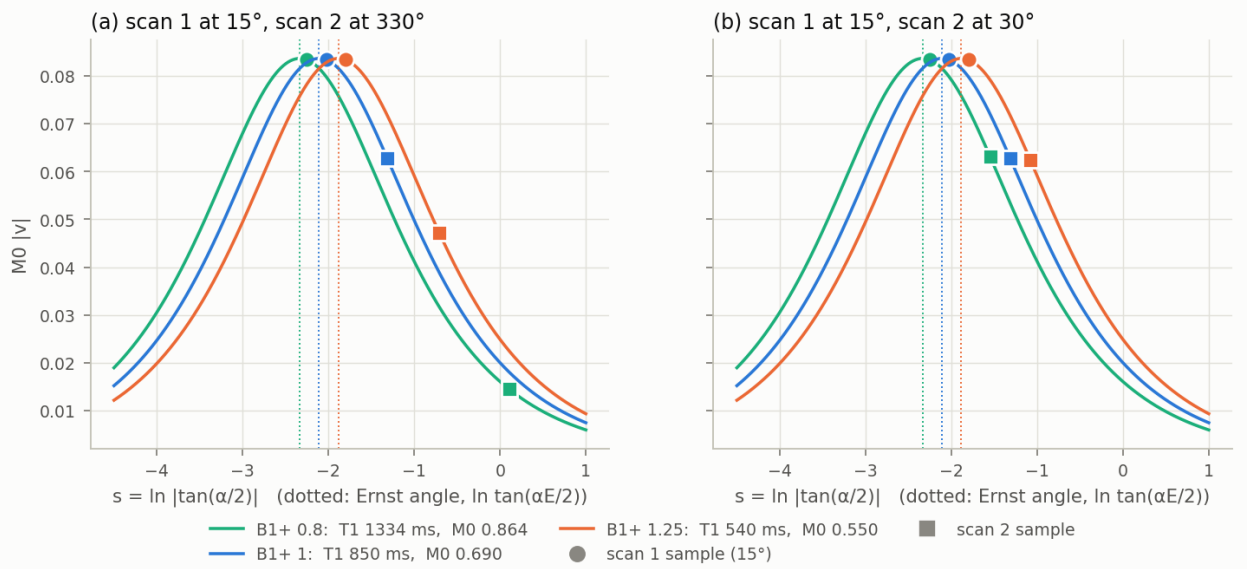
Figure 2: The single-scan degeneracy on the log half-angle axis (WM, T_R = 25 ms). Curves: the amplitude M_0|v| = M_0\zeta \operatorname{sech}(s - s_E) for three members of the family (16) ( B_1^{+'} = 0.8, 1, 1.25 ); dotted lines: their Ernst angles s_E . Circles: the 15^\circ scan-1 sample of each member, at the same offset from its bump and the same height, hence identical scan-1 data. Squares: the scan-2 sample. (a) For 330^\circ the scan-2 samples land at different heights (and, for B_1^{+'} = 1.25 , with the opposite sign of v ). (b) For 30^\circ they almost coincide: a second small flip angle hardly separates the members.
