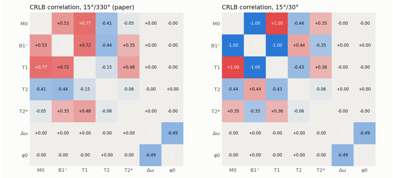
Figure 1: Correlation matrices of the CRLB covariance \mathcal{I}^{-1} . Right: the M_0 – B_1^+ – T_1 block of the small-angle protocol is perfectly correlated, the signature of the invariance (16).
