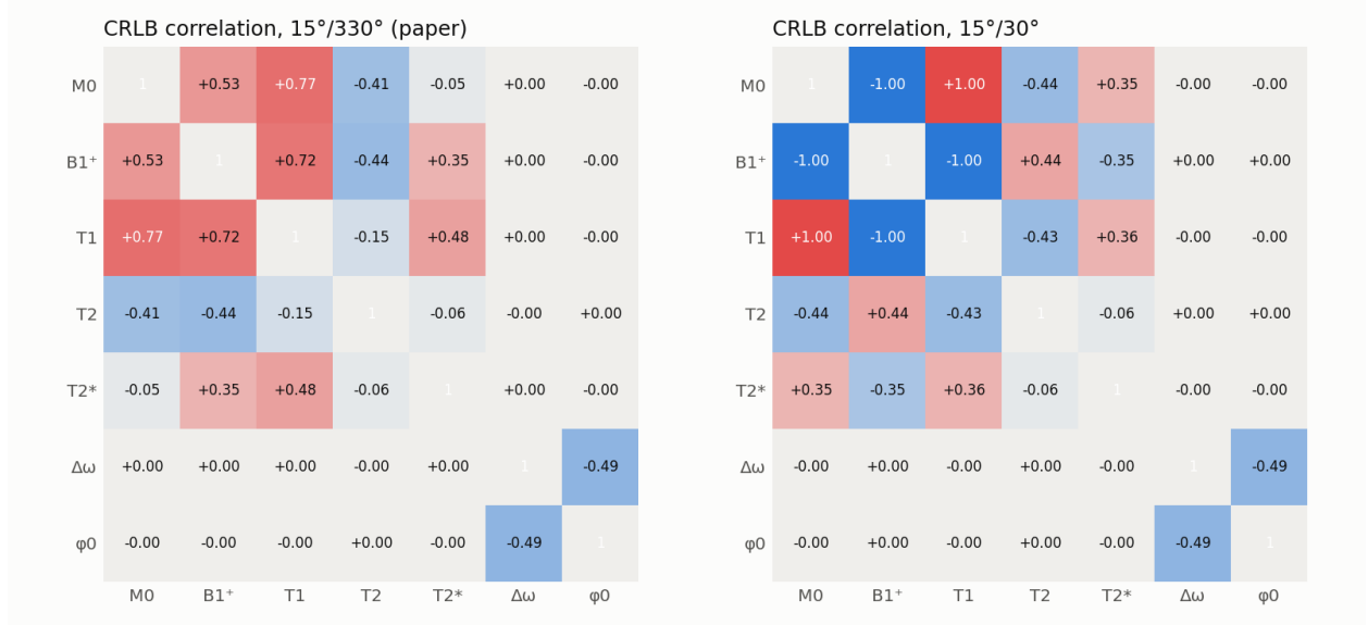
Figure 3: Correlation matrices of \mathcal{I}^{-1} . The M_0 - B_1^+ - T_1 block of the small-angle protocol is perfectly correlated, the signature of (21).
