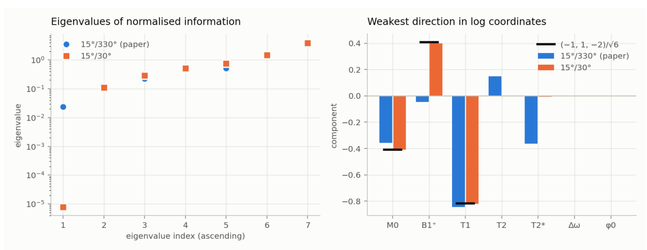
Figure 4: Left: eigenvalues of \tilde{\mathcal{I}} . Right: the weakest direction in log coordinates, w \propto D^{-1/2}u . For 15°/30° it is the symmetry direction (-1, 1, -2)/\sqrt{6} (black); for 15°/330° it is dominated by T_1 (-0.85), with M_0 and T_2^* (-0.36 each), and its B_1^+ component is only -0.05.
