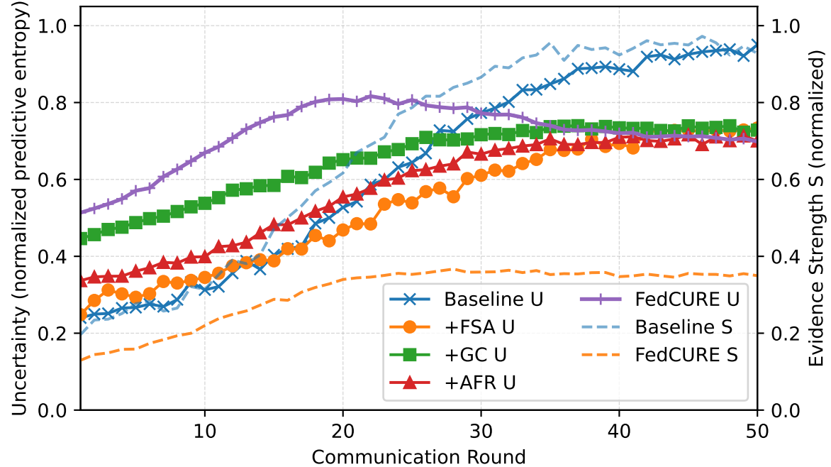
Uncertainty explosion vs. FedCURE rectification
