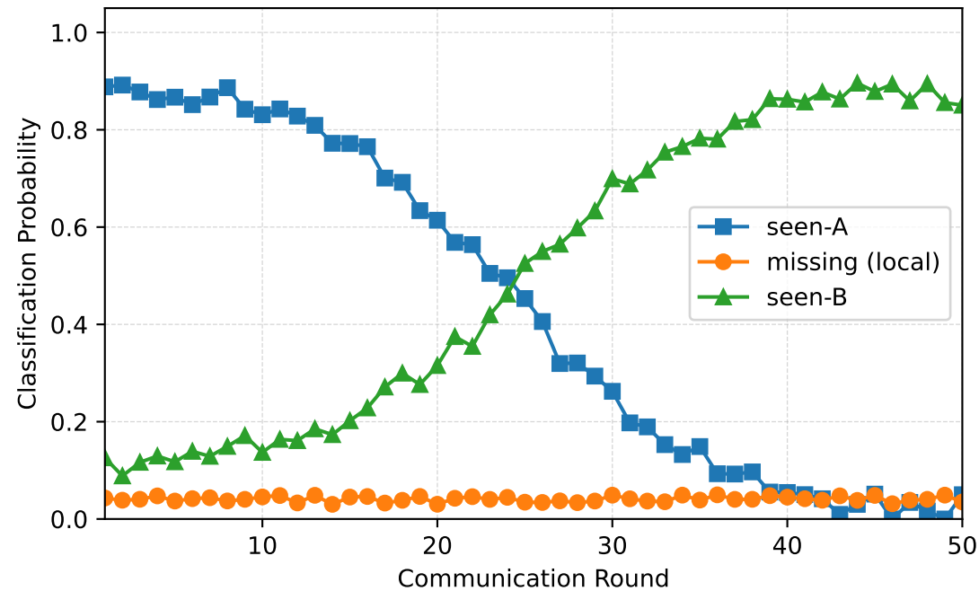
Missing-label client (Baseline EDL): class probabilities
