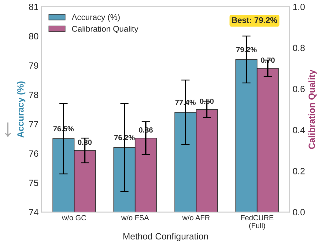
Component Ablation Study
