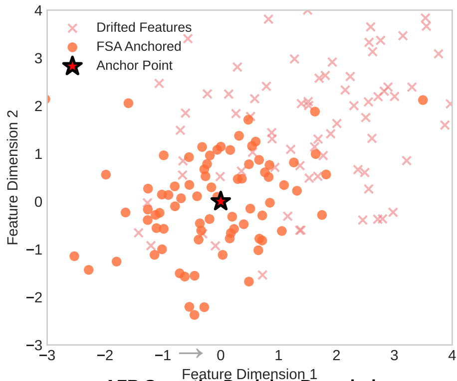
AFR Smooths Decision Boundaries
