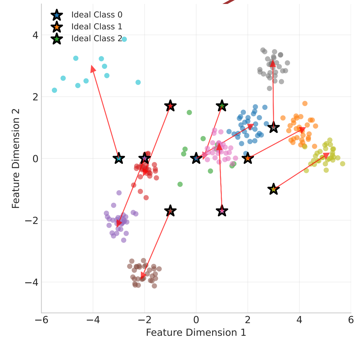
(b) Missing FSA: Feature Representation Drift
