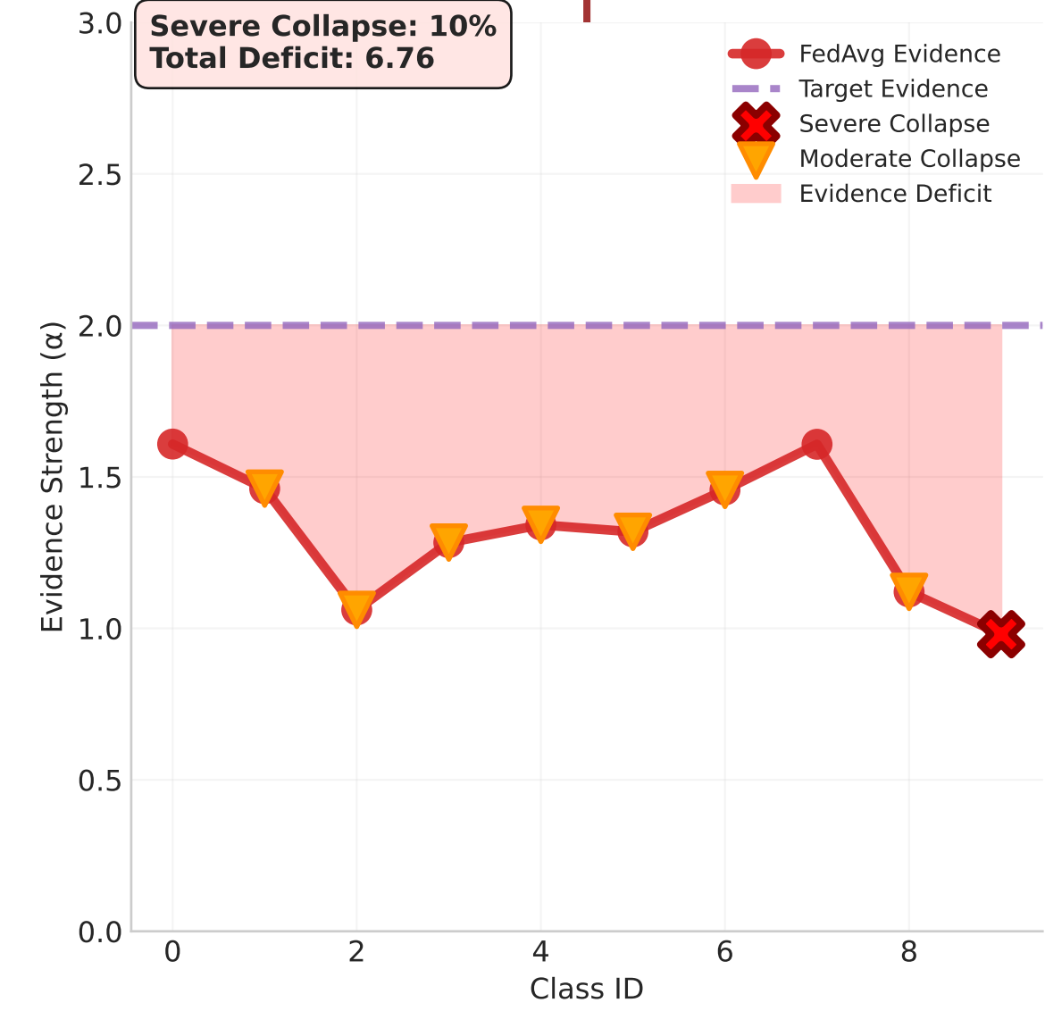
(c) Missing GC: Global Evidence Collapse
