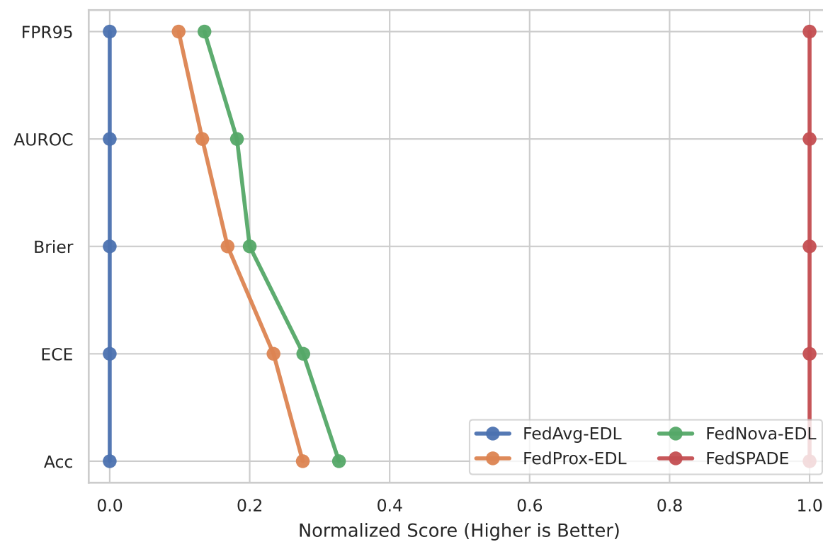
(c) Against Stabilizing EDL Baselines
