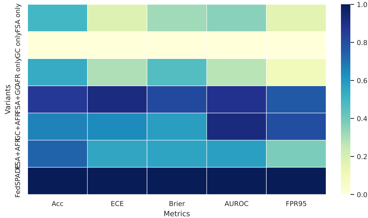
(a) Component Ablation: Unified Metric Score
