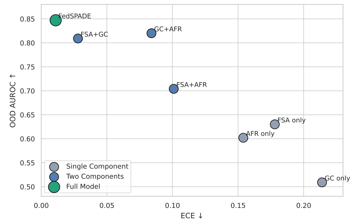
(b) Calibration-OOD Pareto View
