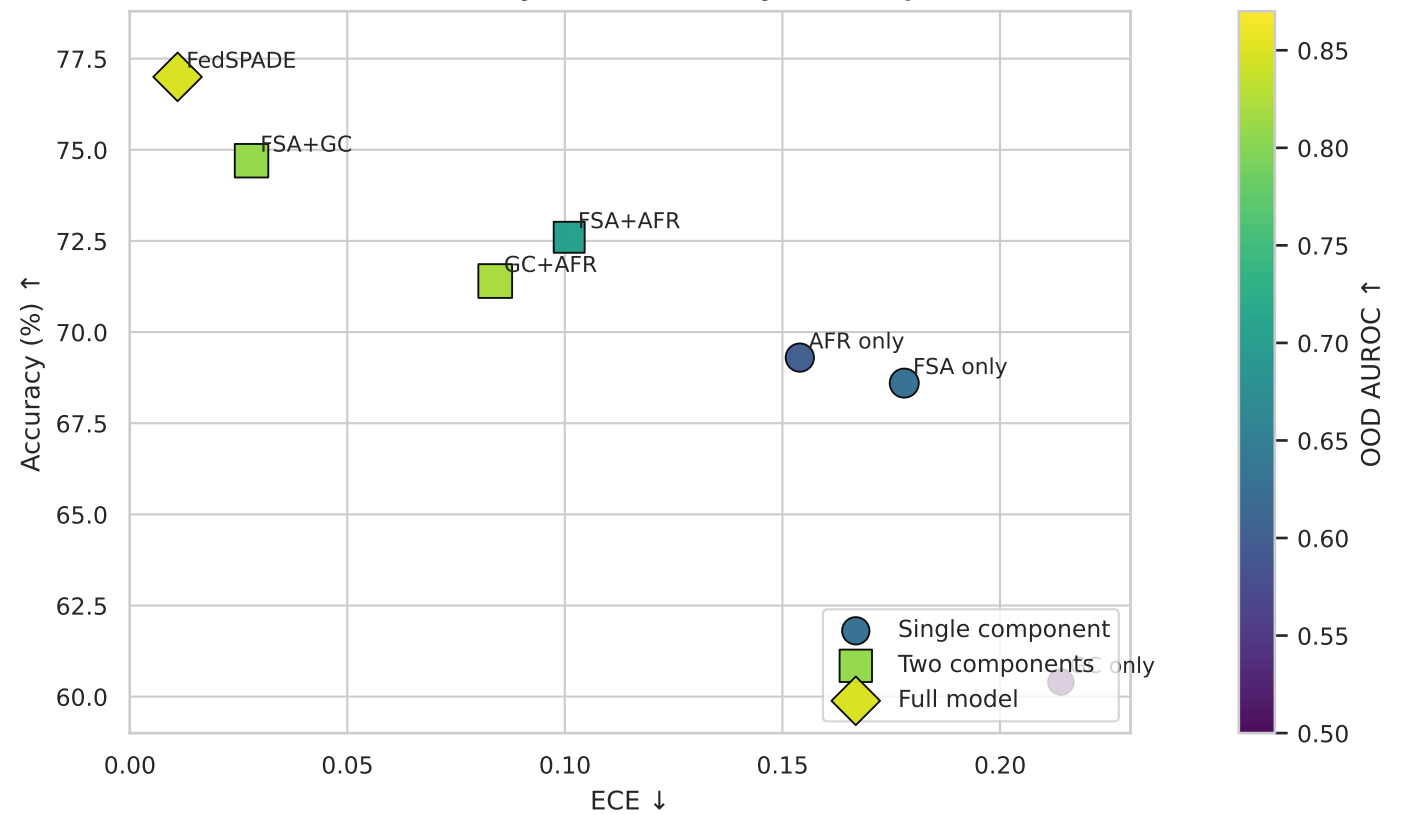
(c) Uncertainty-Aware Accuracy Landscape
