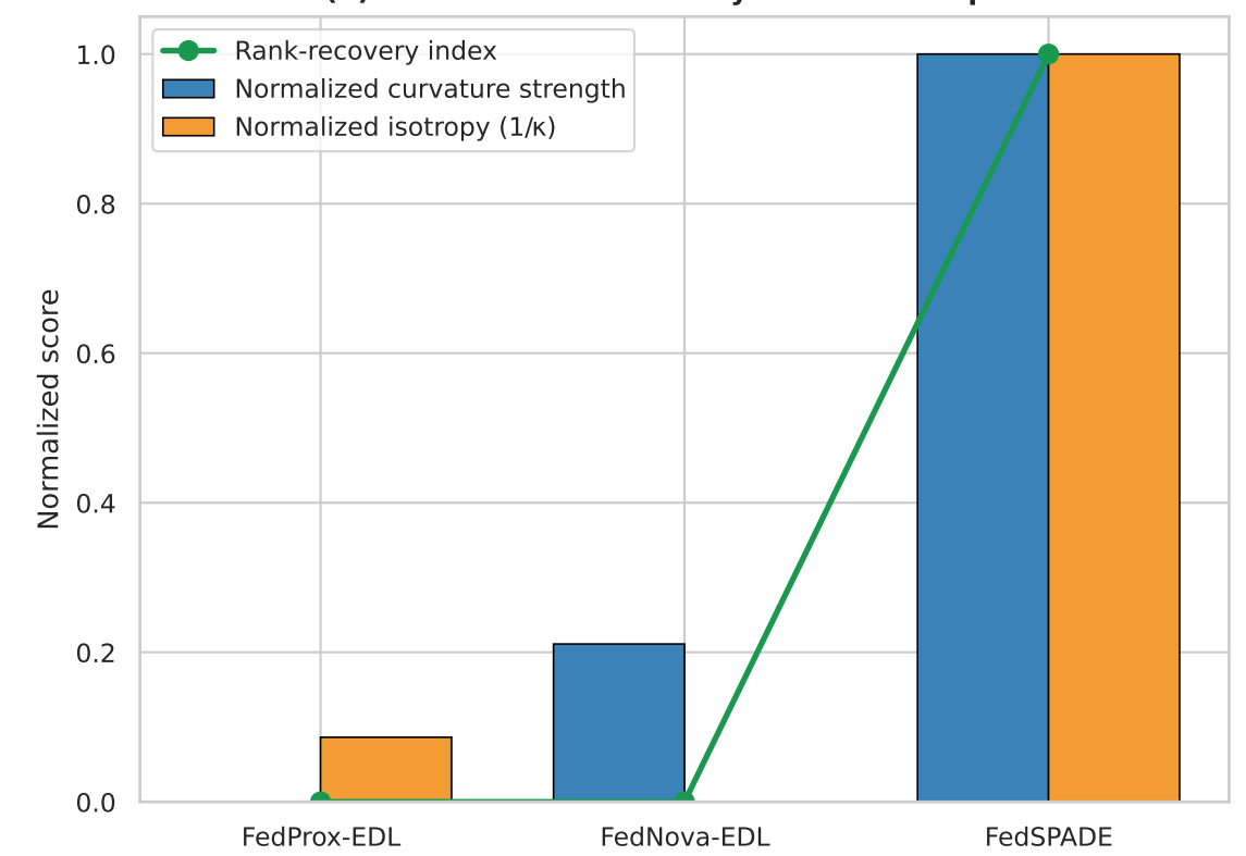
(b) Rank-Balance Recovery in Evidence Space
