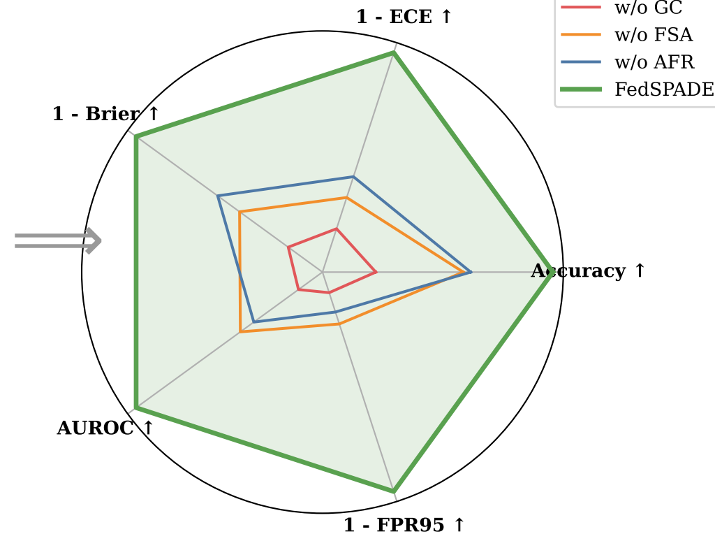
Phase 4: Final Reliability Gap (Ablation Radar Chart)
