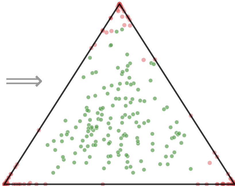
Phase 2: Rank Recovery (Evidence Dirichlet Simplex)
