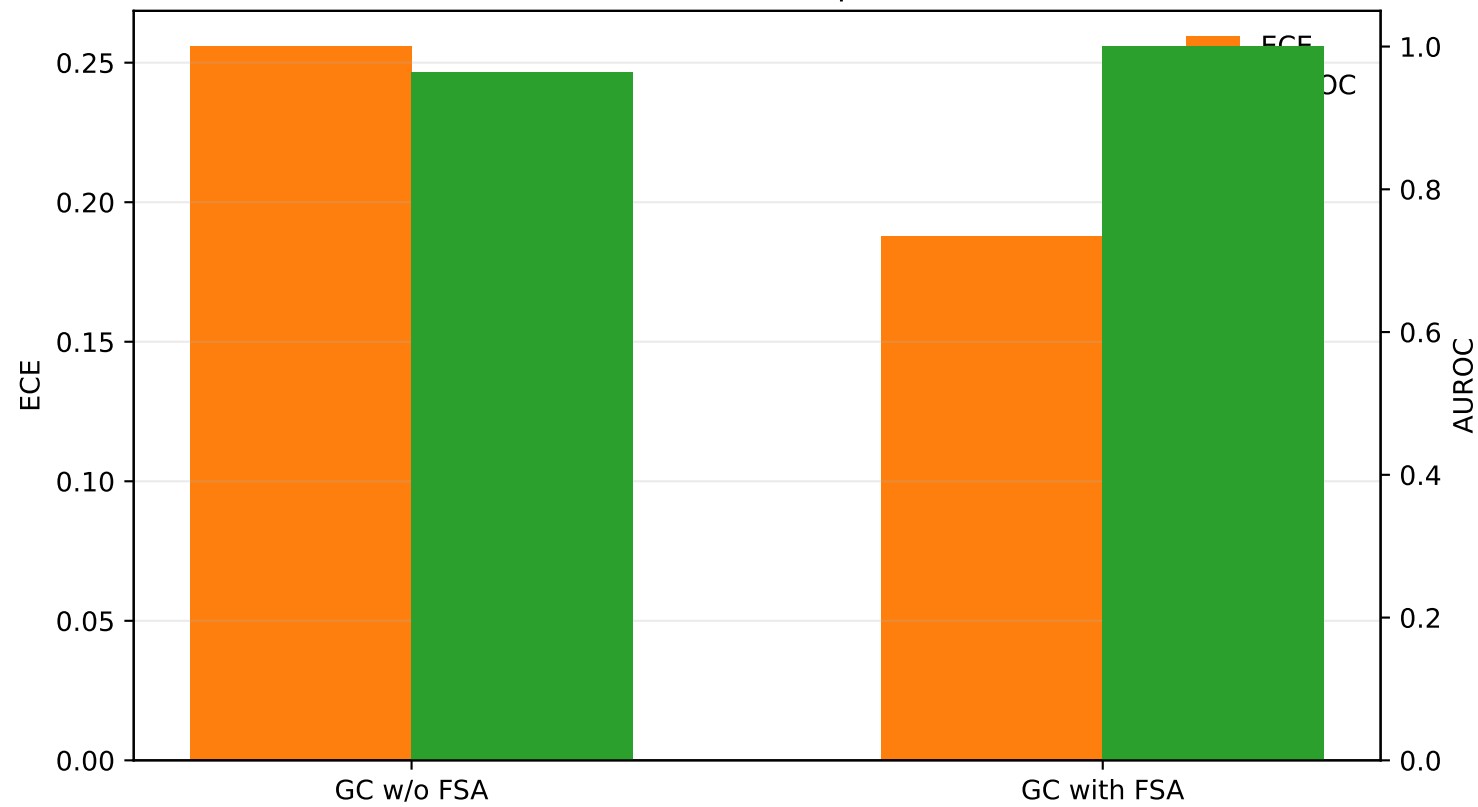
(c) GC Effectiveness Depends on FSA
