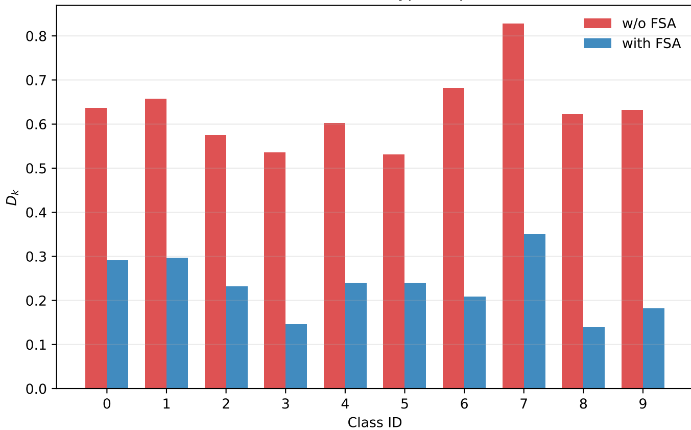
(a) Class-wise Prototype Dispersion
