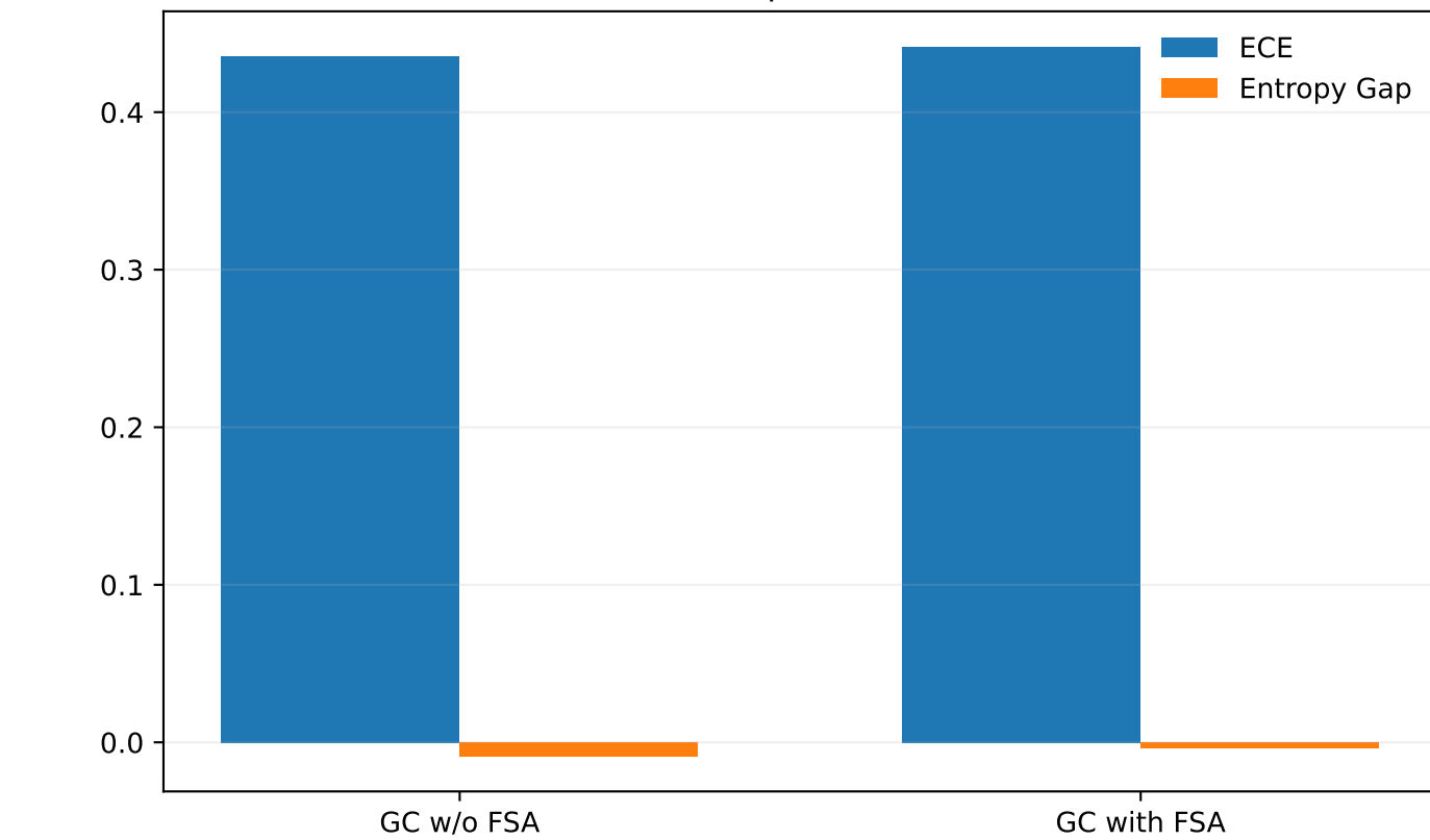
(c) GC Depends on FSA
