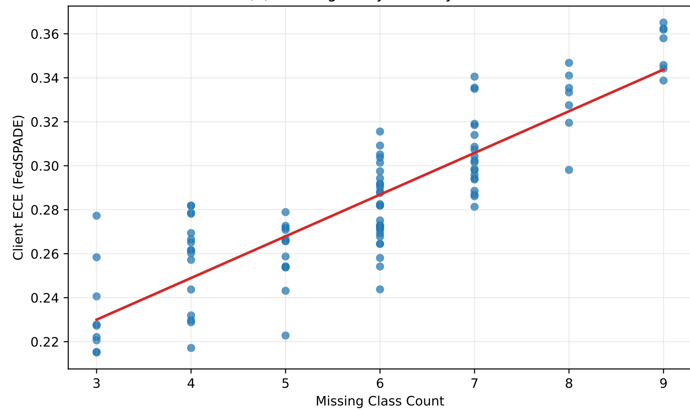
(b) Heterogeneity Severity vs ECE
