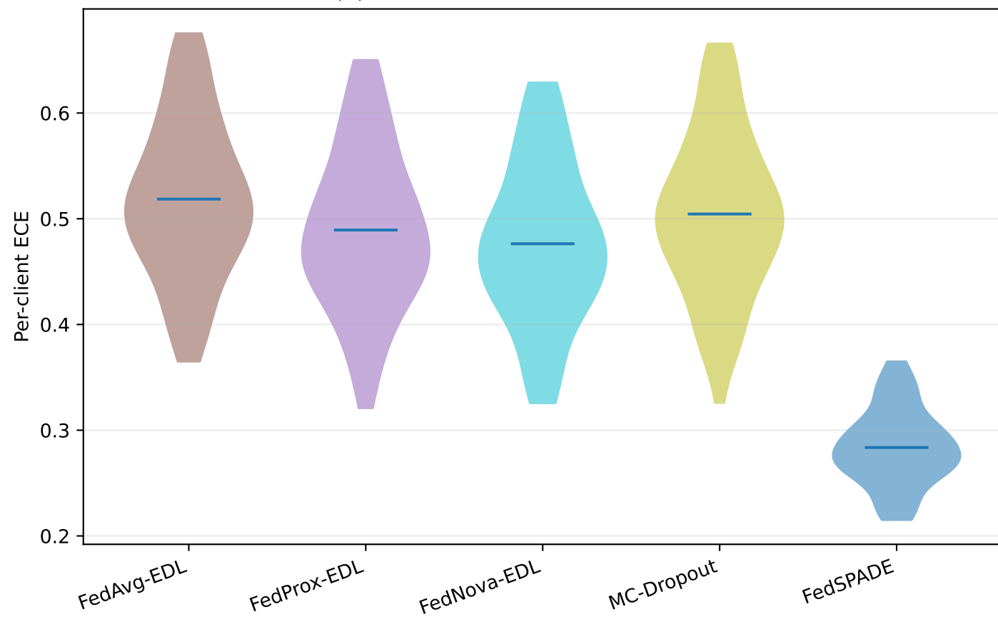
(a) Per-client Calibration Distribution
