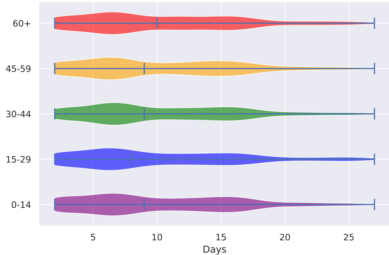
Hospital Days by Age Group (Violin)
