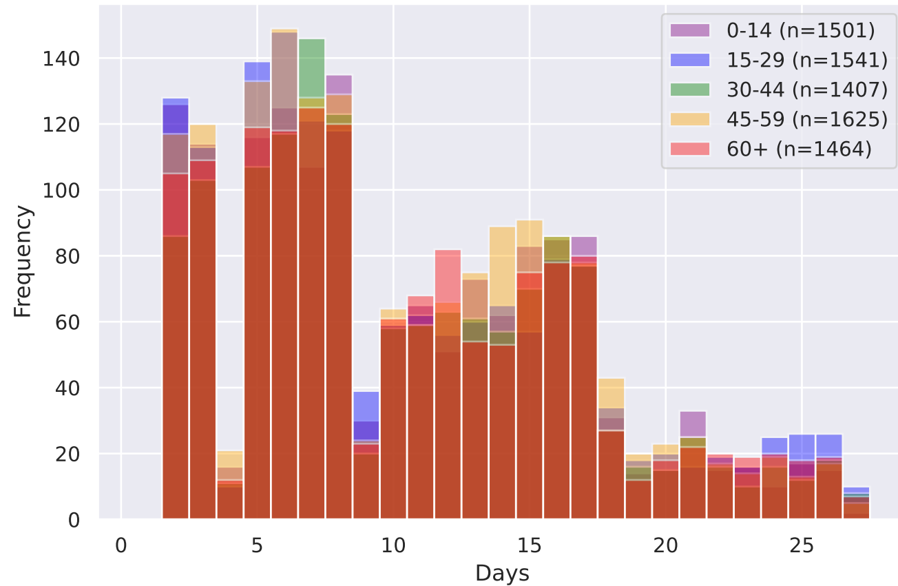
Hospital Days by Age Group
