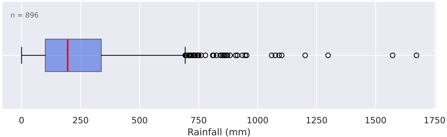
Rainfall — Box Plot
